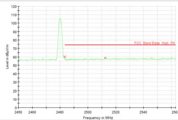
Horizontal / Peak
