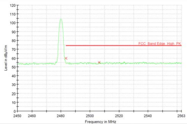
Horizontal / Peak
