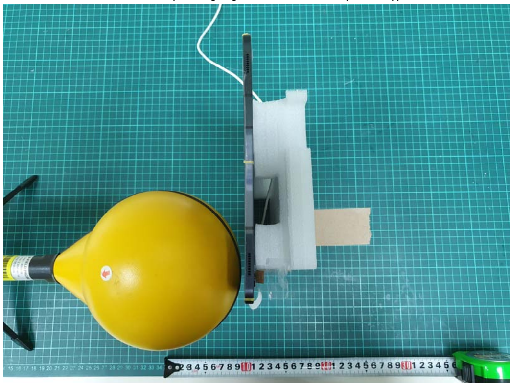
H-Field (Charging Mode - Z-axis (Below))
