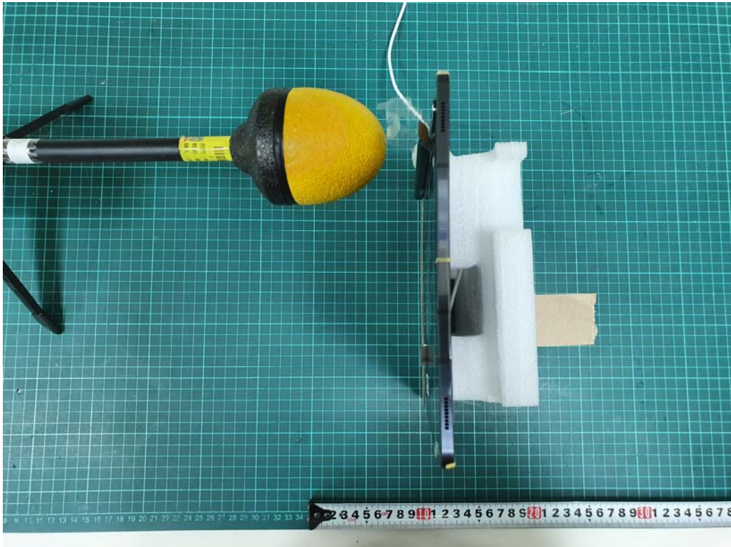
E-Field (Charging Mode - Z-axis (Above))
