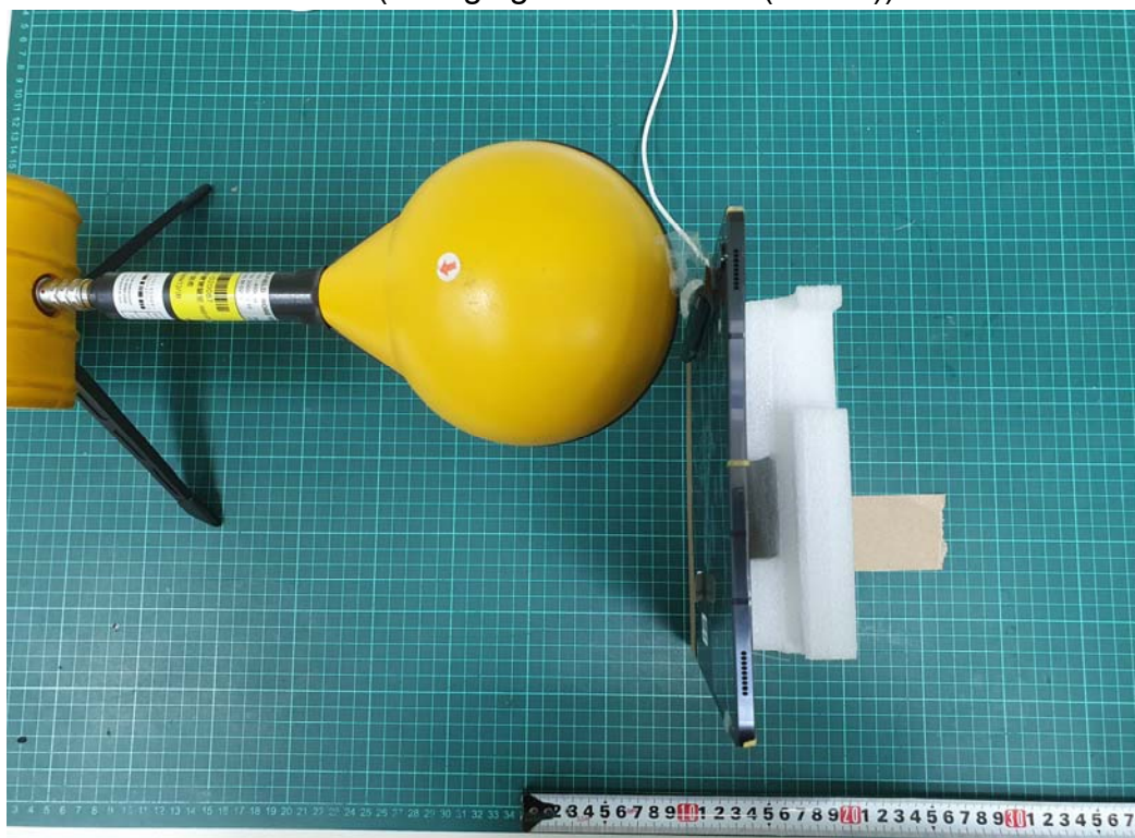
H-Field (Charging Mode - Z-axis (Above))
