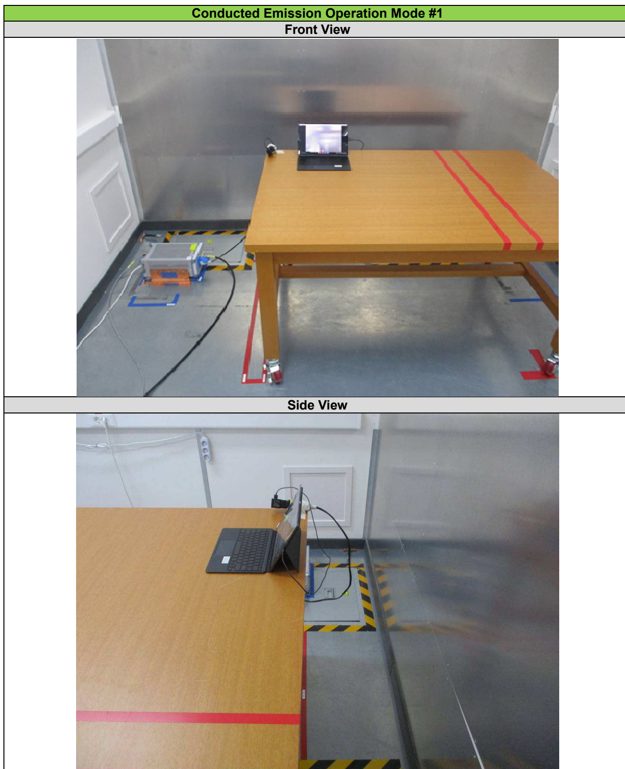
Figure 1. Photo of Conducted emission test setup
