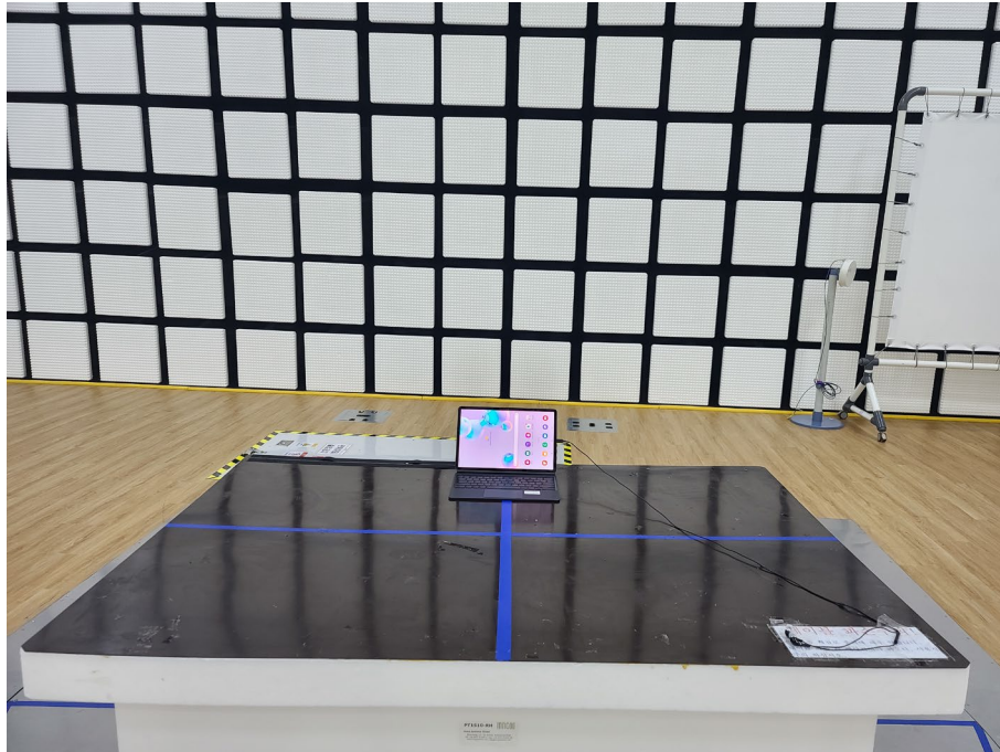
[ Mode 2 - 3 : Front ]
