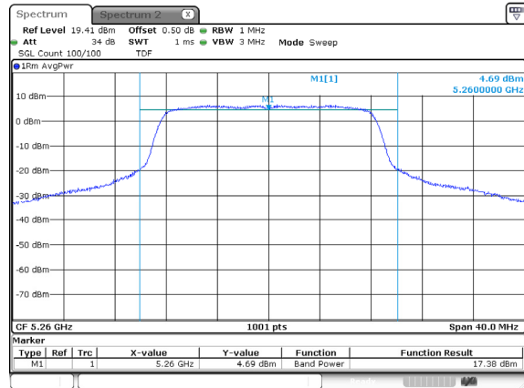
UNII-2A / 802.11a / Mid ch.
