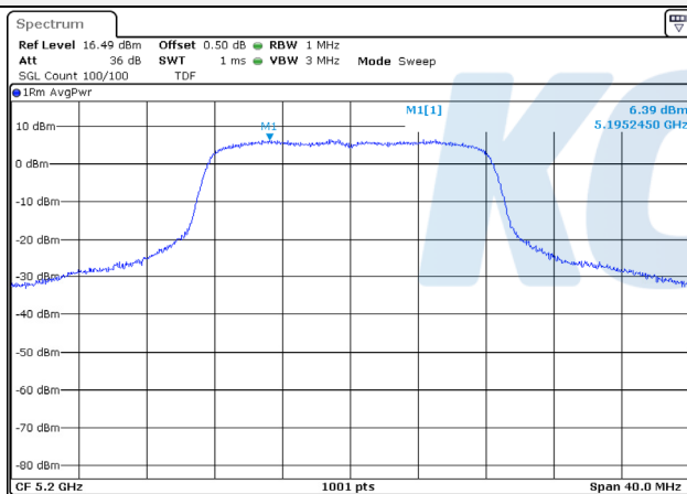
UNII-1 / 802.11a / Mid ch.
