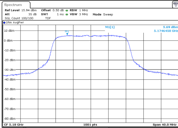
UNII-1 / 802.11a / Low ch.
