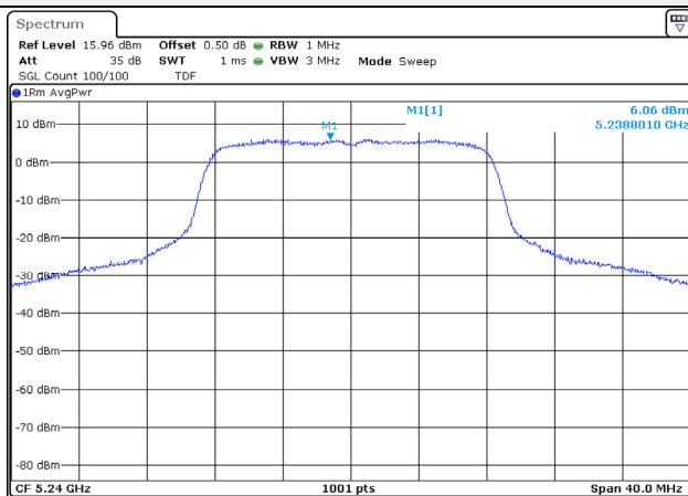
UNII-1 / 802.11a / High ch.
