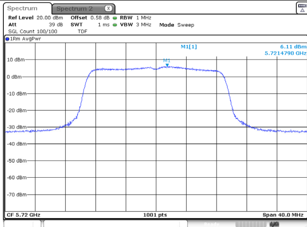
UNII-2C / 802.11n HT40
