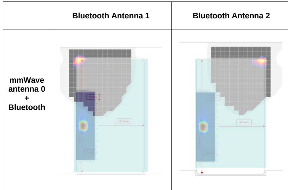
Figure C-2 DUT back side spatial separation of mmWave antenna 0 and Bluetooth antennas
