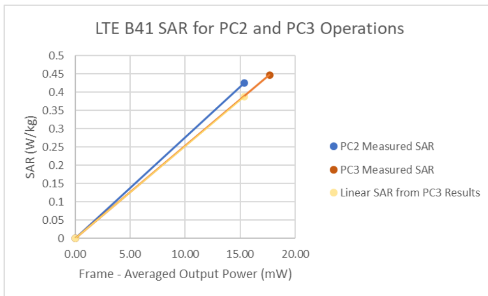
Figure 12-1 LTE Band 41 Body Linearity
