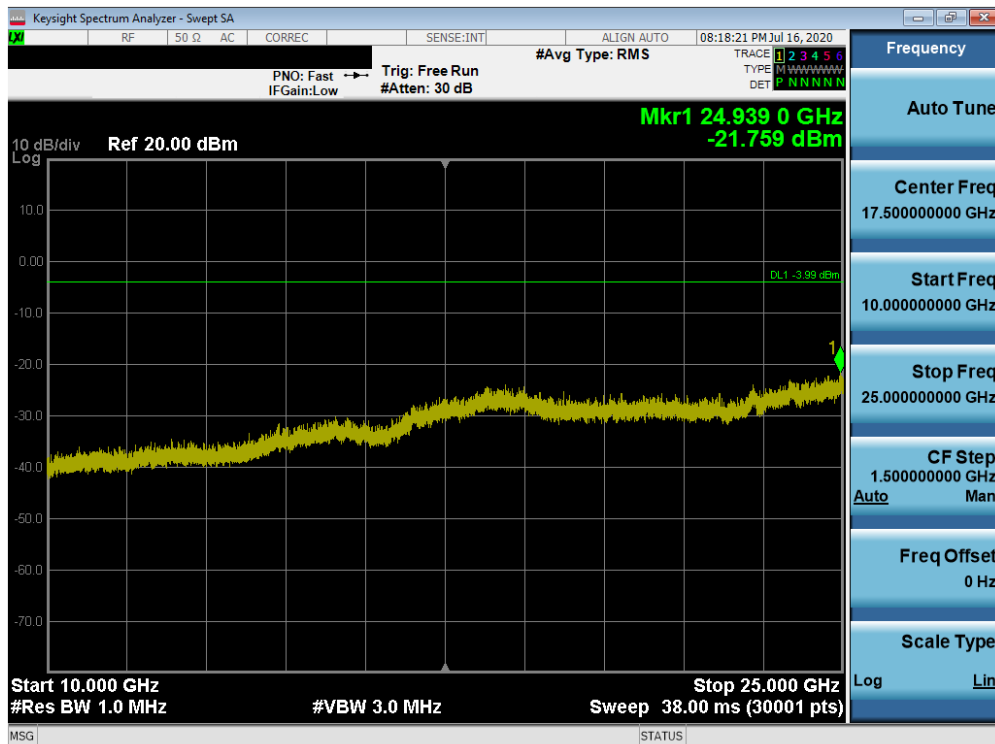
Plot 7-80. Conducted Spurious Plot (Bluetooth, 3Mbps – Ch. 39)
