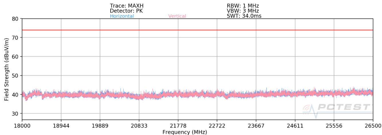
Plot 7-86. Radiated Spurious Plot above 18GHz
