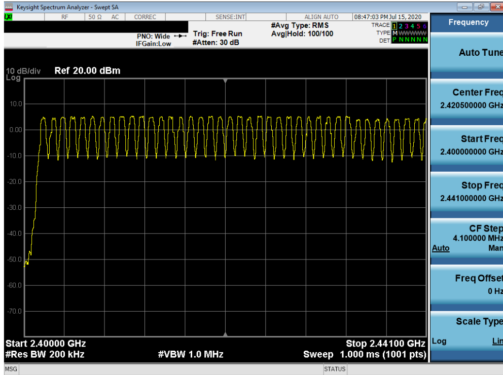
Plot 7-67. Low End Spectrum Channel Hopping Plot (Bluetooth) – ANT0
