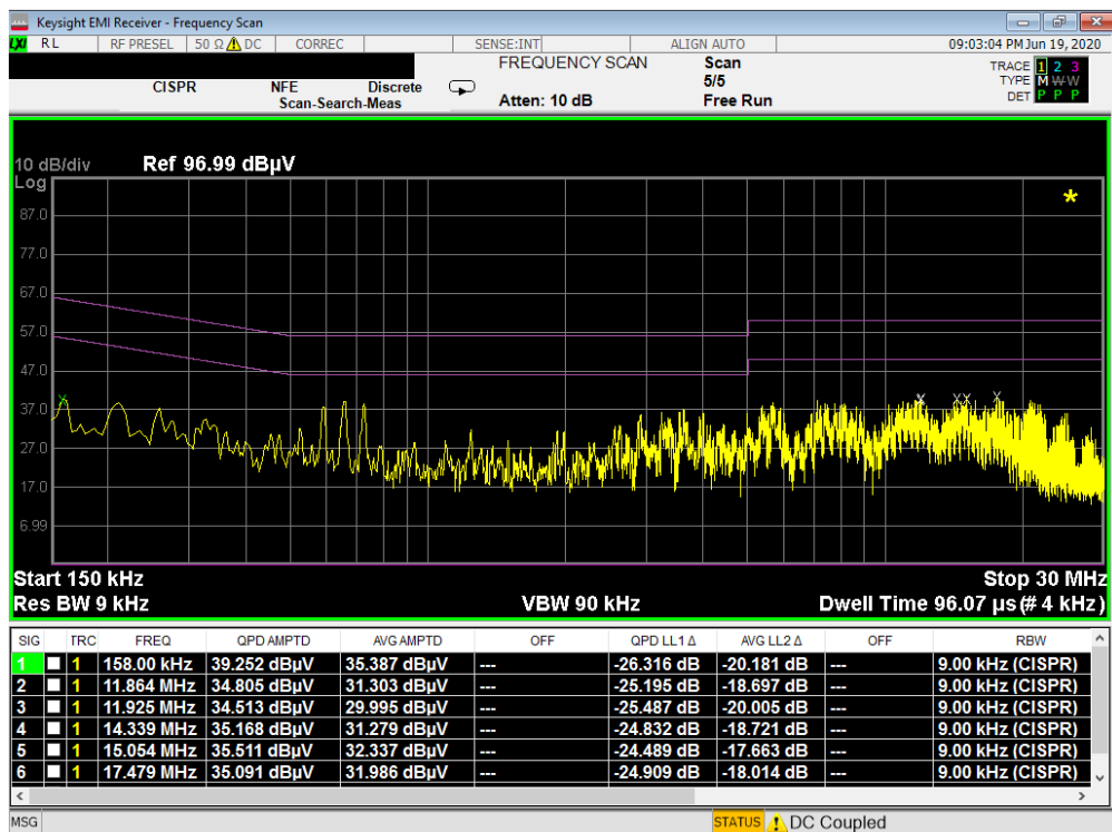
Plot 7-98. Line-Conducted Test Plot (N) – ANT0
