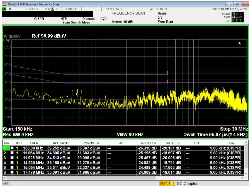
Plot 7-100. Line-Conducted Test Plot (N) – ANT1
