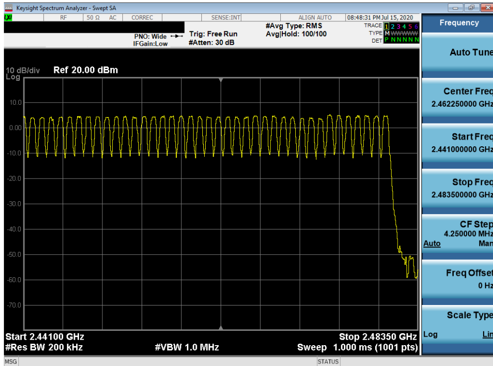
Plot 7-68. High End Spectrum Channel Hopping Plot (Bluetooth) – ANT0
