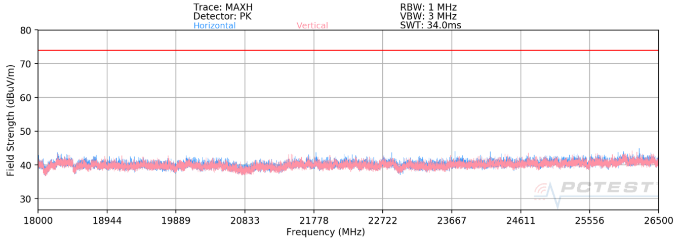
Plot 7-90. Radiated Spurious Plot above 18GHz
