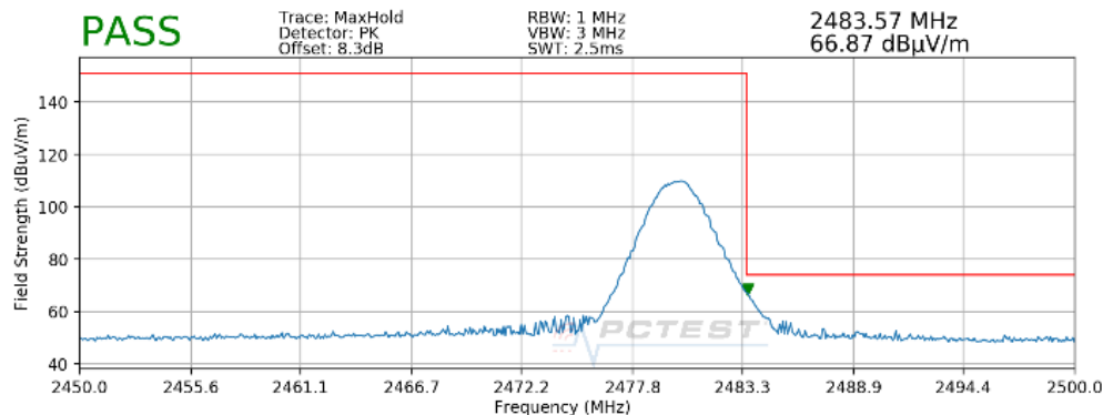
Plot 7-94. Radiated Restricted Upper Band Edge Measurement (Peak)
