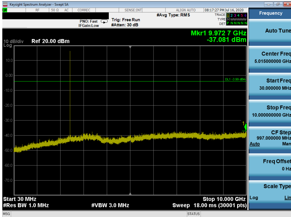
Plot 7-79. Conducted Spurious Plot (Bluetooth, 3Mbps – Ch. 39)
