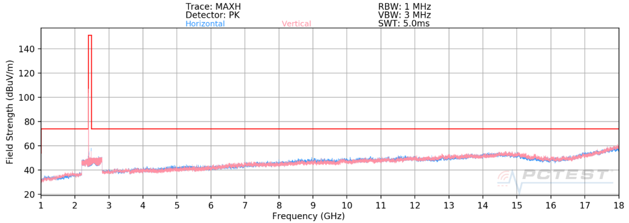
Plot 7-87. Radiated Spurious Plot above 1GHz (BT- Ch. 0)
