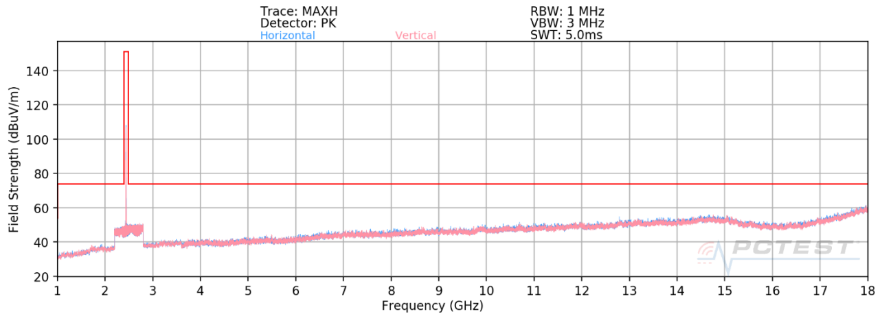
Plot 7-88. Radiated Spurious Plot above 1GHz (BT- Ch. 39)
