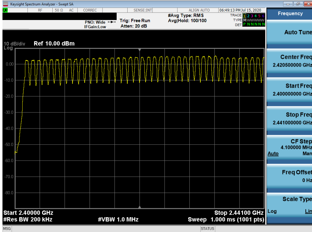
Plot 7-69. Low End Spectrum Channel Hopping Plot (Bluetooth) – ANT1
