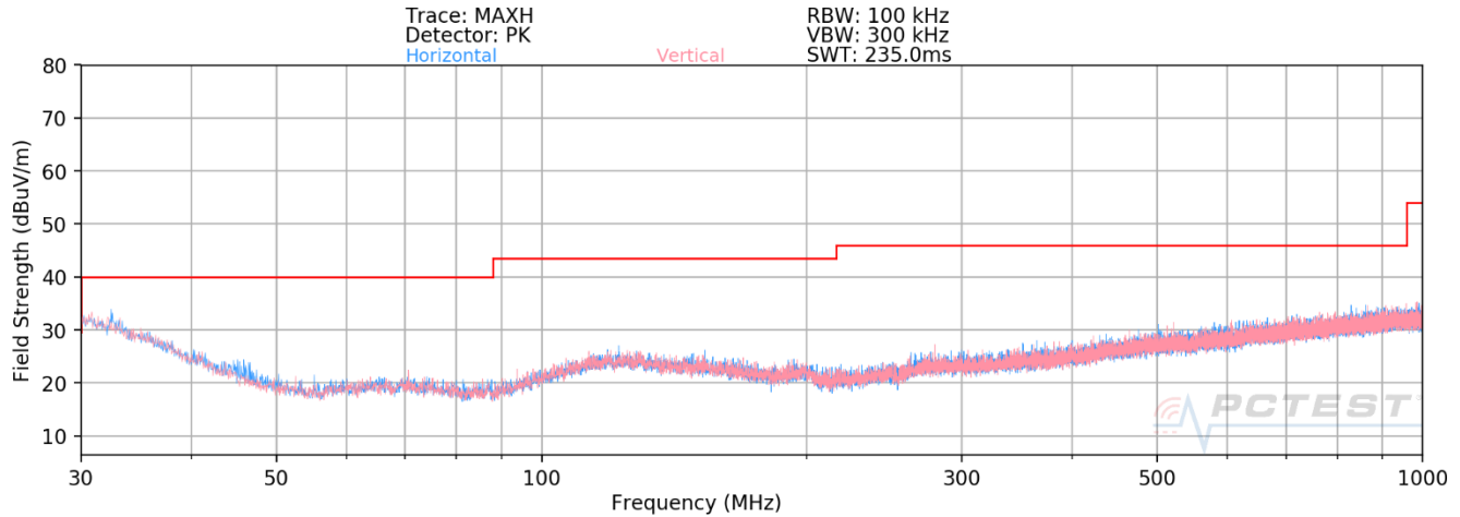
Plot 7-95. Radiated Spurious Plot below 1GHz – ANT0
