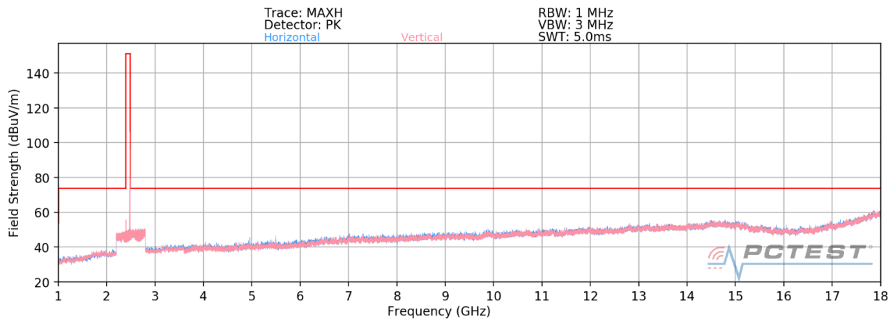
Plot 7-89. Radiated Spurious Plot above 1GHz (BT- Ch. 78)
