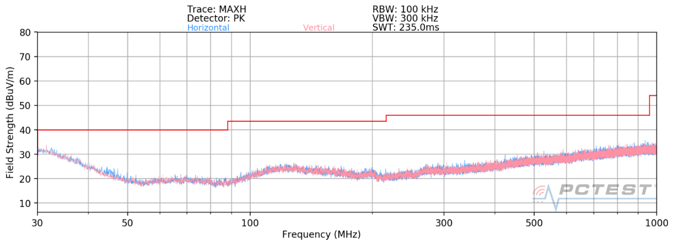
Plot 7-96. Radiated Spurious Plot below 1GHz – ANT1
