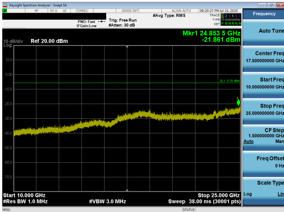
Plot 7-82. Conducted Spurious Plot (Bluetooth, 3Mbps – Ch. 78)
