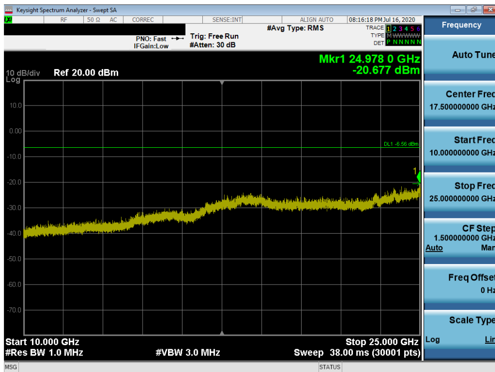
Plot 7-78. Conducted Spurious Plot (Bluetooth, 3Mbps – Ch. 0)
