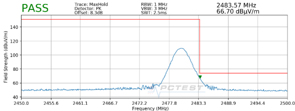
Plot 7-92. Radiated Restricted Upper Band Edge Measurement (Peak)
