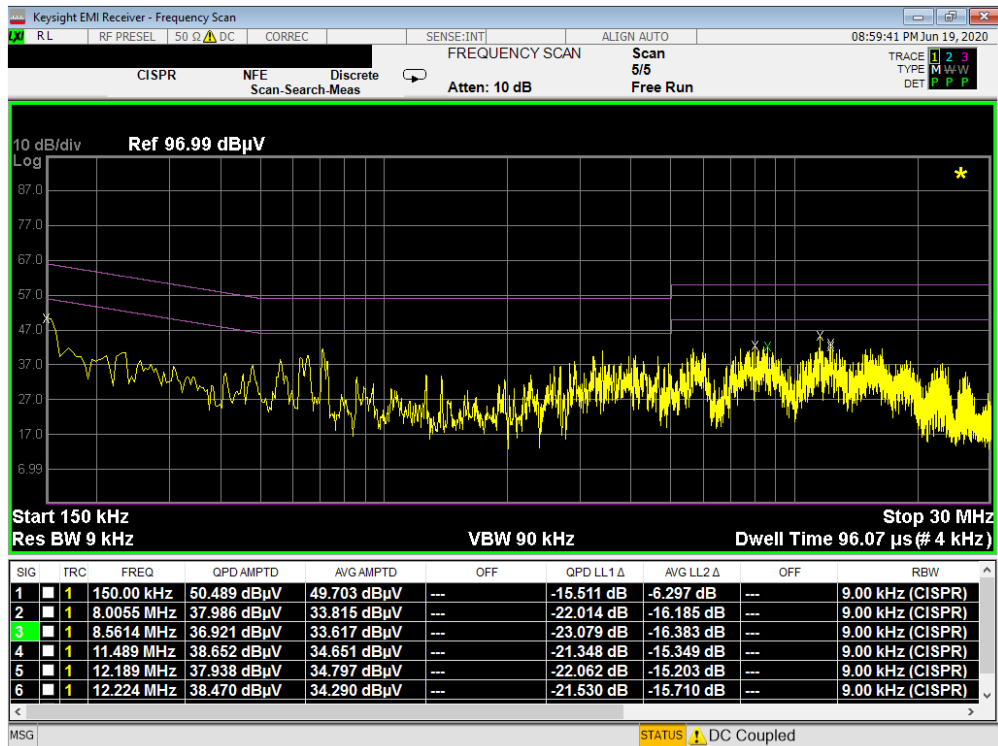
Plot 7-97. Line-Conducted Test Plot (L1) – ANT0
