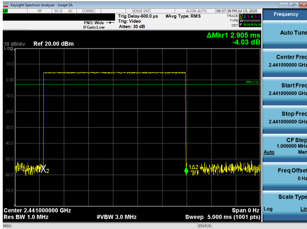
Plot 7-65. Time of Occupancy Plot (Bluetooth) – ANT0
