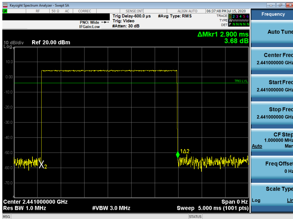
Plot 7-66. Time of Occupancy Plot (Bluetooth) – ANT1
