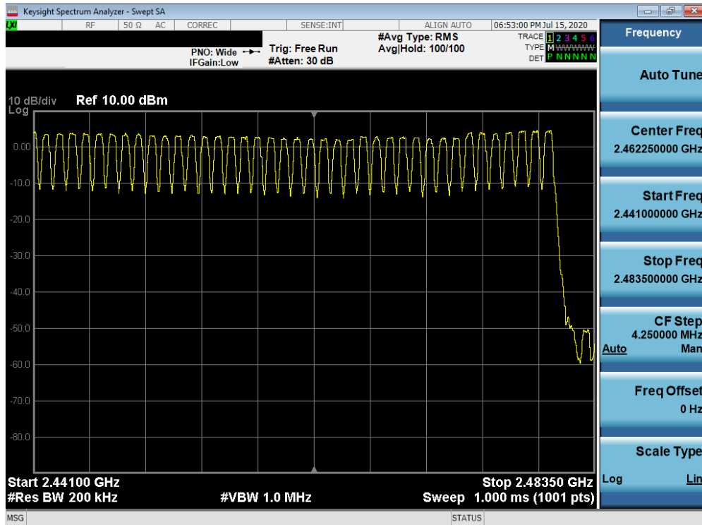
Plot 7-70. High End Spectrum Channel Hopping Plot (Bluetooth) – ANT1
