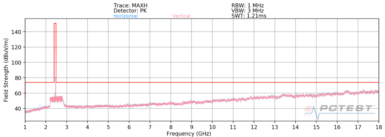
Plot 7-85. Radiated Spurious Plot above 1GHz (BT- Ch. 78)
