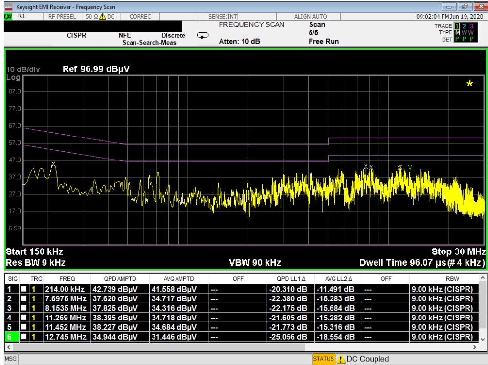
Plot 7-99. Line-Conducted Test Plot (L1) – ANT1
