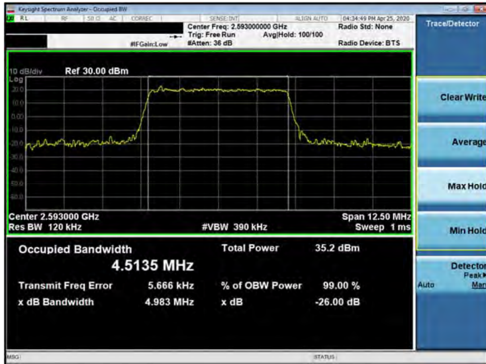
Plot 7-205. Occupied Bandwidth Plot (Band 41 (PC2) - 5.0MHz QPSK - Full RB Configuration)
