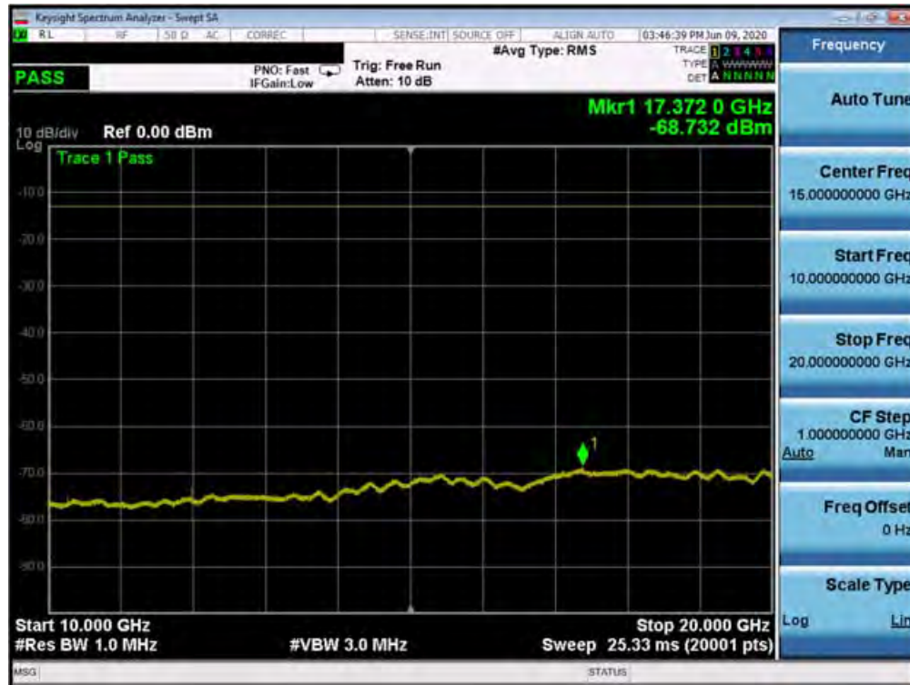
Plot 7-315. Conducted Spurious Plot (n66 - 20MHz DFT-s-OFDM-QPSK - RB Size 1, RB Offset 1 - Low Channel)
