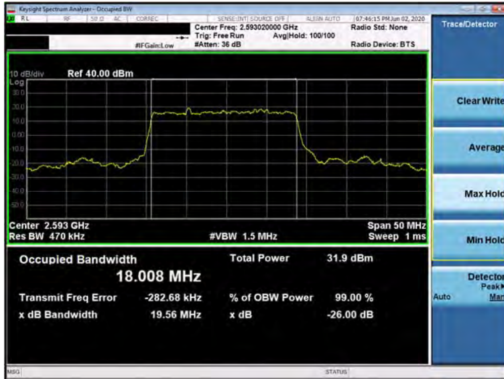
Plot 7-221. Occupied Bandwidth Plot (n41 20MHz BPSK-DFT-s-OFDM - Full RB Configuration)
