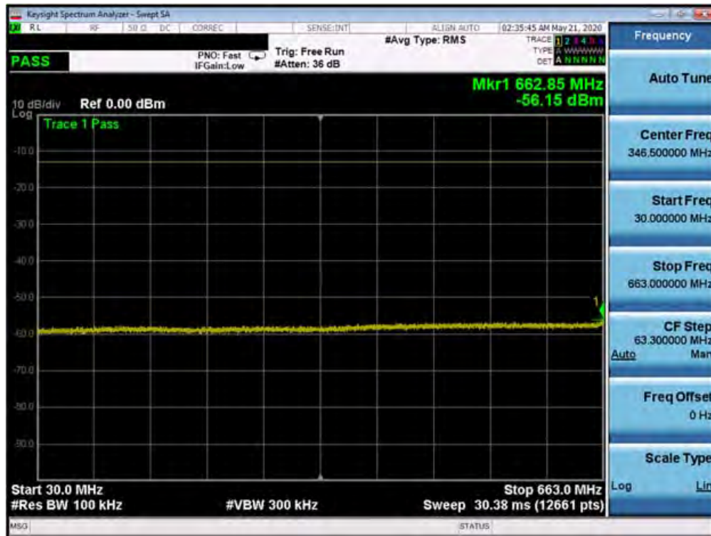
Plot 7-265. Conducted Spurious Plot (n71 - 20MHz DFT-s-OFDM-QPSK - RB Size 1, RB Offset 1 - Low Channel)
