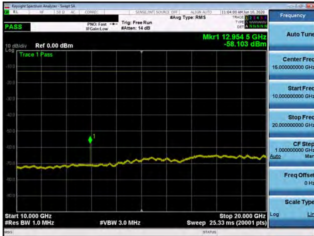
Plot 7-333. Conducted Spurious Plot (n25/2 - 20MHz DFT-s-OFDM-QPSK - RB Size 1, RB Offset 1 - Low Channel)
