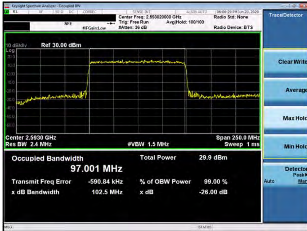
Plot 7-253. Occupied Bandwidth Plot (n41 100MHz 16QAM-CP-OFDM - Full RB Configuration)
