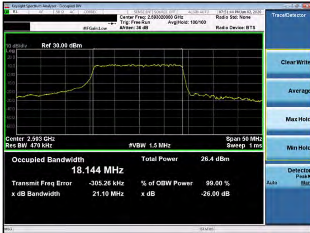
Plot 7-225. Occupied Bandwidth Plot (n41 20MHz 256QAM-CP-OFDM- Full RB Configuration)
