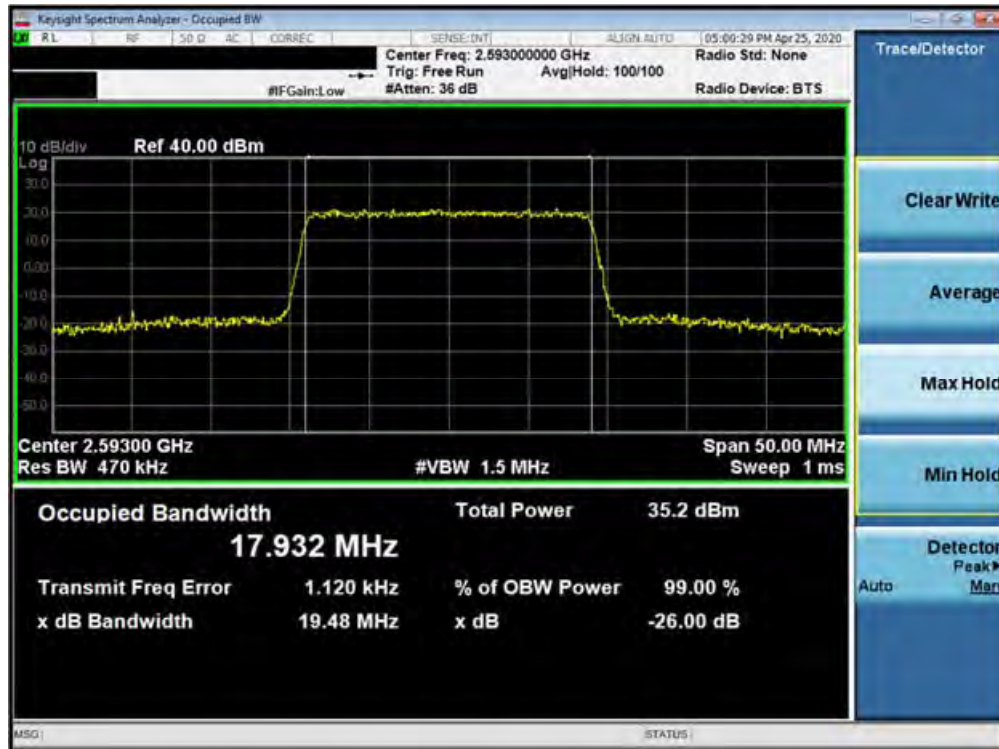
Plot 7-217. Occupied Bandwidth Plot (Band 41 (PC2) - 20.0MHz QPSK - Full RB Configuration)
