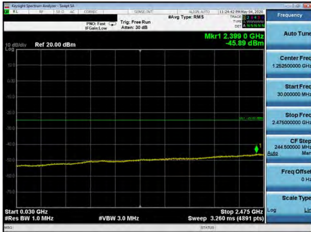
Plot 7-340. Conducted Spurious Plot (Band 7 - 20.0MHz QPSK - RB Size 1, RB Offset 0 - Low Channel)
