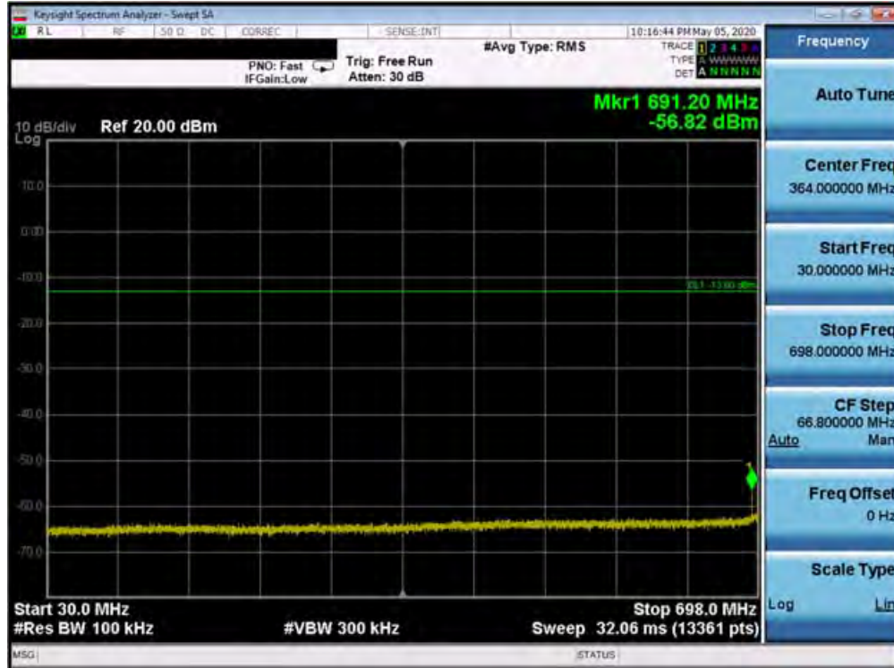
Plot 7-280. Conducted Spurious Plot (Band 12 - 10.0MHz QPSK - RB Size 1, RB Offset 0 - High Channel)
