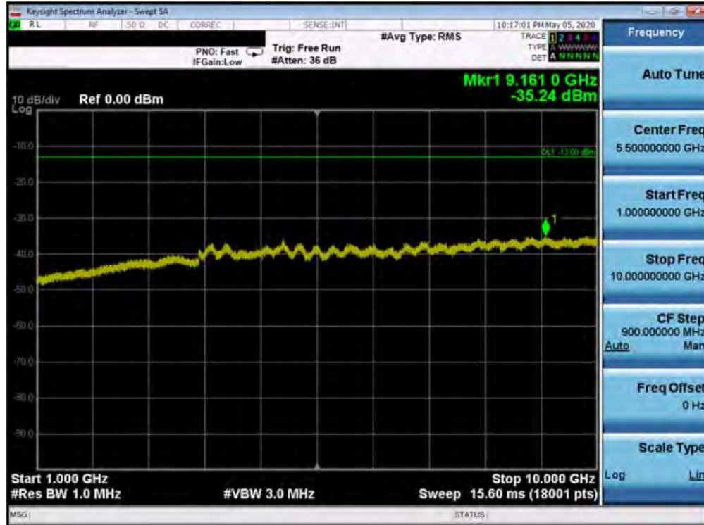
Plot 7-282. Conducted Spurious Plot (Band 12 - 10.0MHz QPSK - RB Size 1, RB Offset 0 - High Channel)
