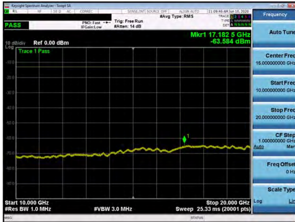
Plot 7-339. Conducted Spurious Plot (n25/2 - 20MHz DFT-s-OFDM-QPSK - RB Size 1, RB Offset 1 - High Channel)
