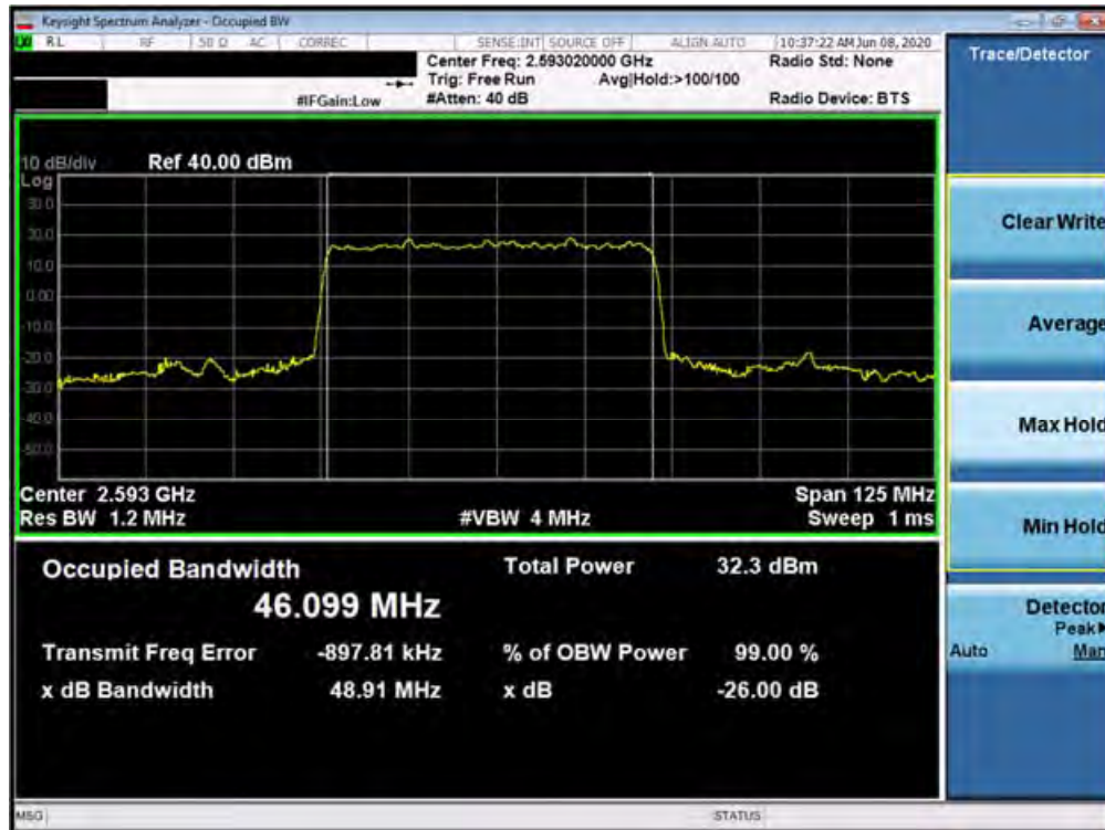
Plot 7-231. Occupied Bandwidth Plot (n41 50MHz BPSK-DFT-s-OFDM - Full RB Configuration)
