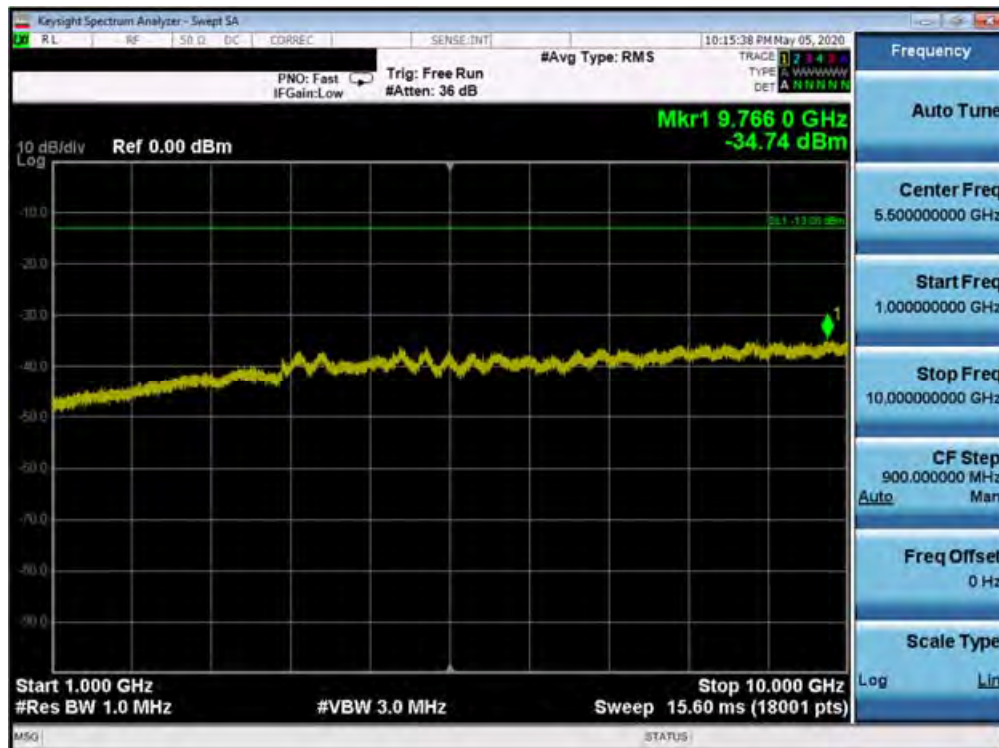
Plot 7-279. Conducted Spurious Plot (Band 12 - 10.0MHz QPSK - RB Size 1, RB Offset 0 - Mid Channel)
