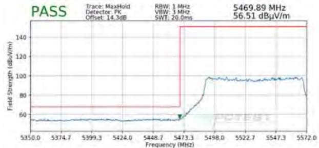
Plot 7-326. Radiated Lower Band Edge Plot SISO ANT1 (Peak – UNII Band 2C – 996 Tones)
