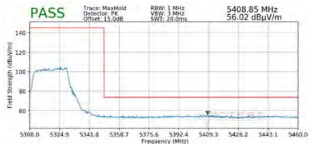
Plot 7-331. Radiated Upper Band Edge Plot SISO ANT2 (Peak - UNII Band 2A - 242 Tones)
