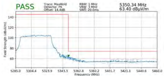
Plot 7-359. Radiated Upper Band Edge Plot MIMO (Peak - UNII Band 2A - 484 Tones)
