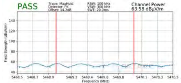
Plot 7-361. Radiated Lower Band Edge Plot MIMO (Peak - UNII Band 2C - 484 Tones)
