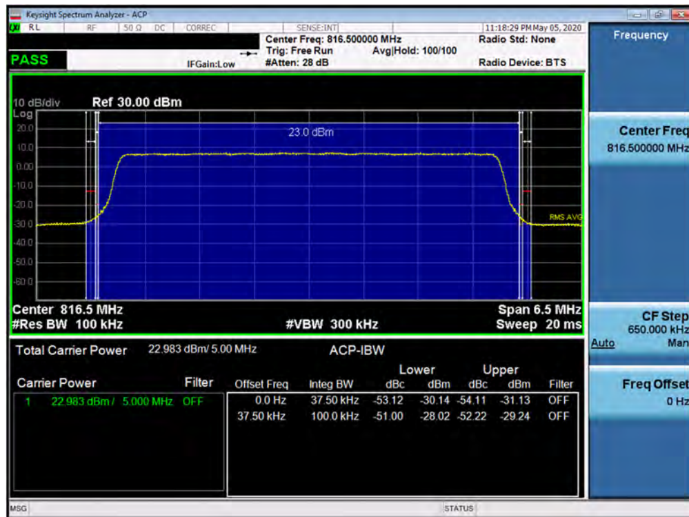
Plot 7-26. Channel Edge Plot (LTE Band 26 - 5MHz QPSK - Low Channel)
