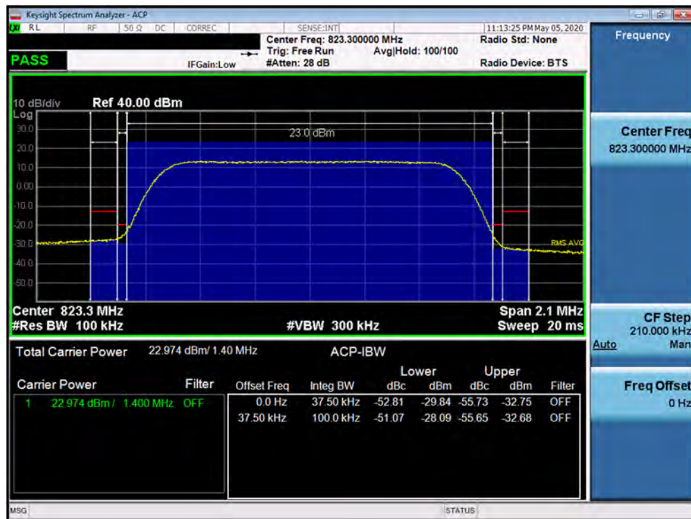
Plot 7-31. Channel Edge Plot (LTE Band 26 - 1.4MHz QPSK - High Channel)
