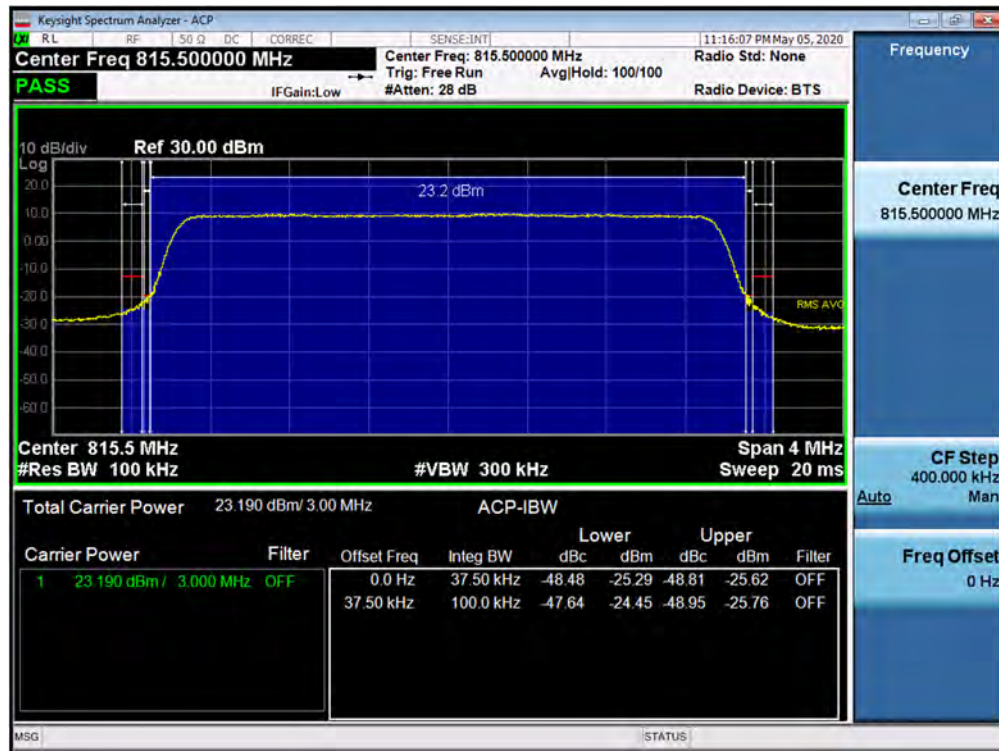
Plot 7-28. Channel Edge Plot (LTE Band 26 - 3MHz QPSK - Low Channel)
