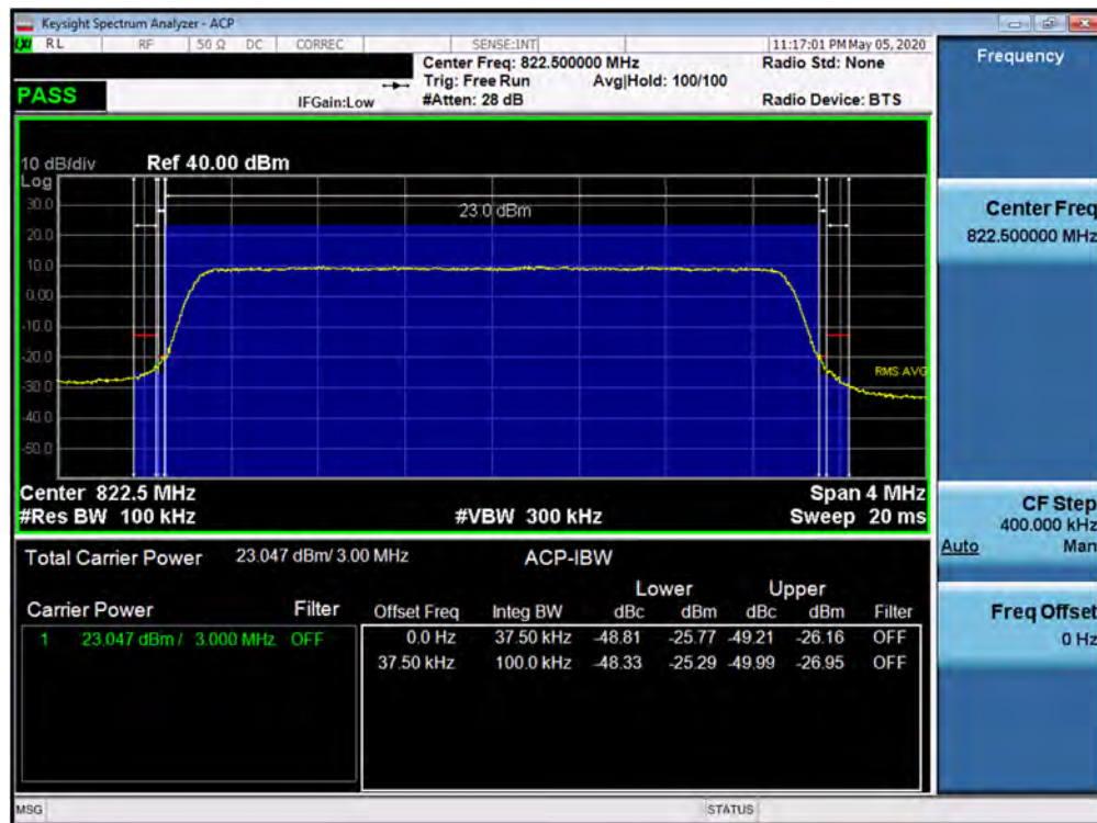
Plot 7-29. Channel Edge Plot (LTE Band 26 - 3MHz QPSK - High Channel)
