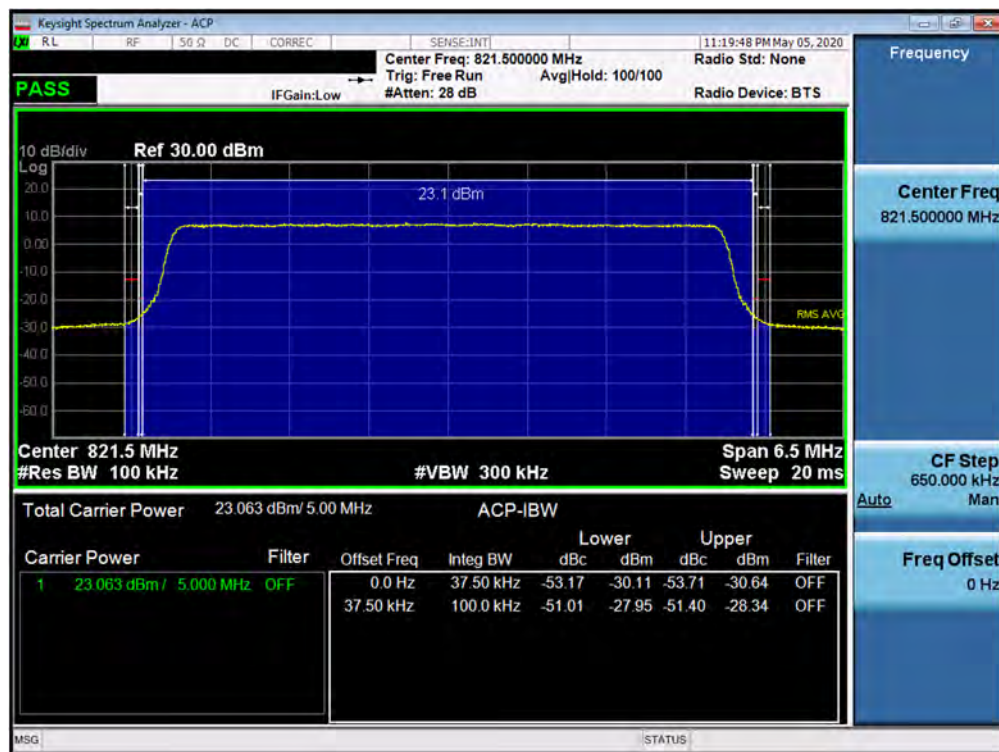
Plot 7-27. Channel Edge Plot (LTE Band 26 - 5MHz QPSK - High Channel)
