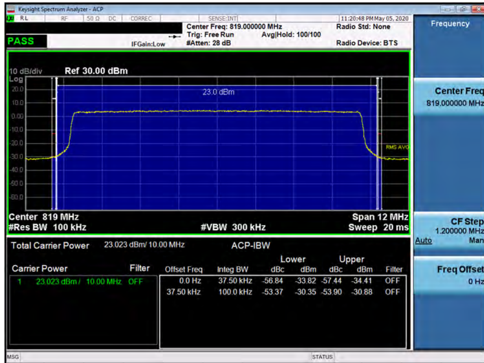
Plot 7-25. Channel Edge Plot (LTE Band 26 - 10MHz QPSK)
