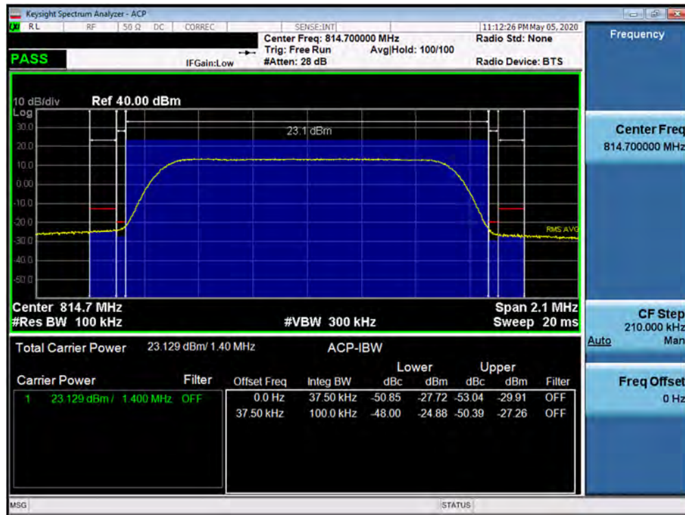
Plot 7-30. Channel Edge Plot (LTE Band 26 - 1.4MHz QPSK - Low Channel)
