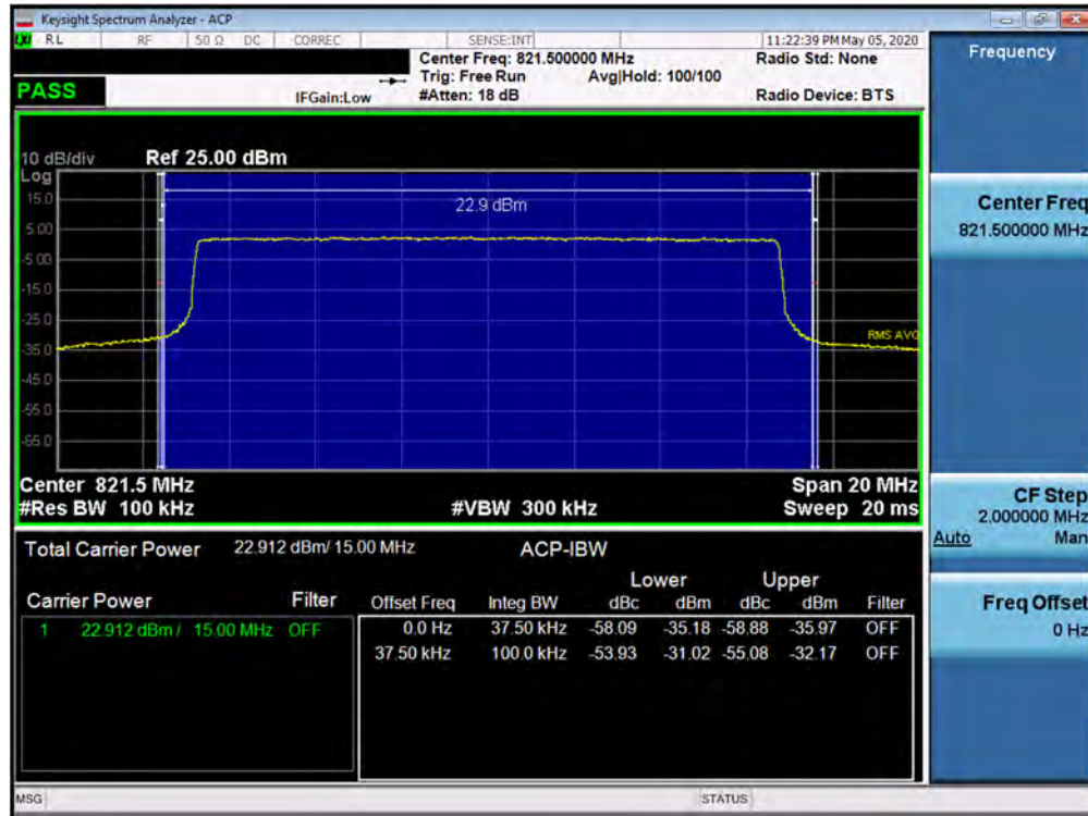
Plot 7-24. Channel Edge Plot (LTE Band 26 - 15MHz QPSK)
