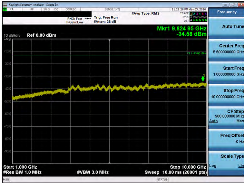
Plot 7-23. Conducted Spurious Plot (LTE Band 26 - 15MHz QPSK - RB Size 1, RB Offset 0)
