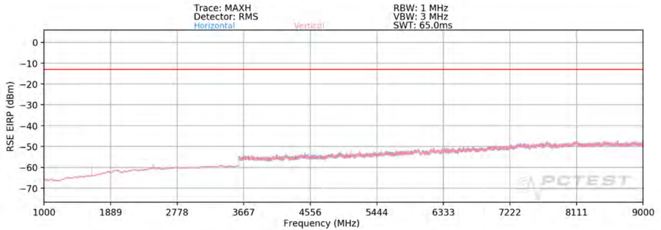
Plot 7-33. Radiated Spurious Plot (Band 26)
