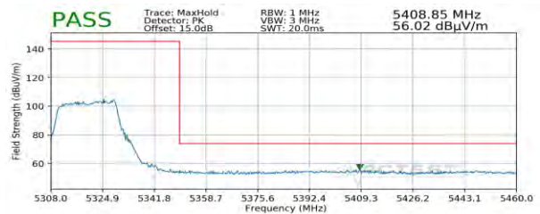
Plot 7-310. Radiated Upper Band Edge Plot SISO ANT2 (Peak – UNII Band 2A)
