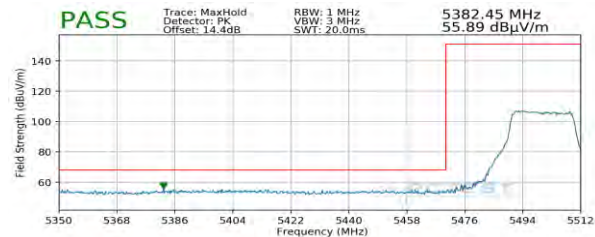
Plot 7-333. Radiated Lower Band Edge Plot MIMO (Peak – UNII Band 2C)
