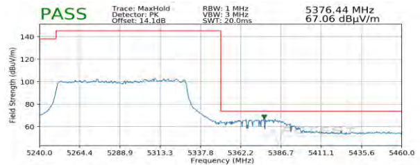
Plot 7-303. Radiated Upper Band Edge Plot SISO ANT1 (Peak – UNII Band 2A)
