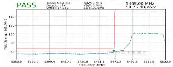
Plot 7-319. Radiated Lower Band Edge Plot SISO ANT2 (Peak – UNII Band 2C)
