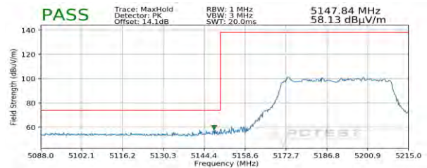
Plot 7-315. Radiated Lower Band Edge Plot SISO ANT2 (Peak – UNII Band 1)
