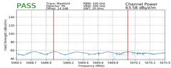
Plot 7-340. Radiated Lower Band Edge Plot MIMO (Peak – UNII Band 2C)
