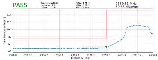
Plot 7-130. Radiated Restricted Lower Band Edge Measurement SISO ANT2 (Peak)
