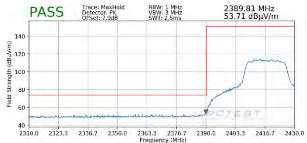
Plot 7-138. Radiated Restricted Lower Band Edge Measurement MIMO (Peak)
