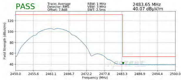
Plot 7-119. Radiated Restricted Upper Band Edge Measurement SISO ANT1 (Average)
