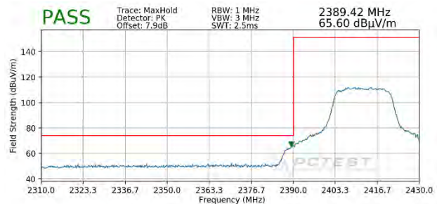
Plot 7-136. Radiated Restricted Lower Band Edge Measurement MIMO (Peak)
