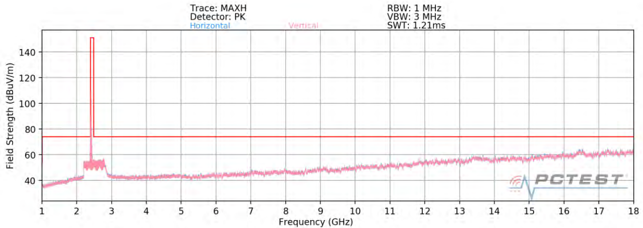
Plot 7-107. Radiated Spurious Plot above 1GHz SISO ANT2 (802.11b – Ch. 1)
