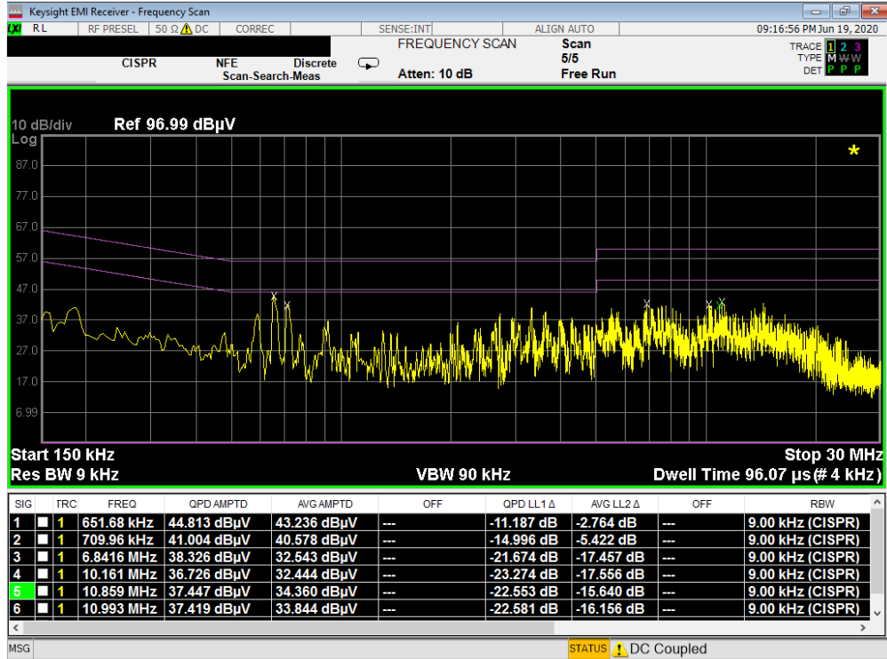
Plot 7-144. Line Conducted Plot with 802.11b (L1)
