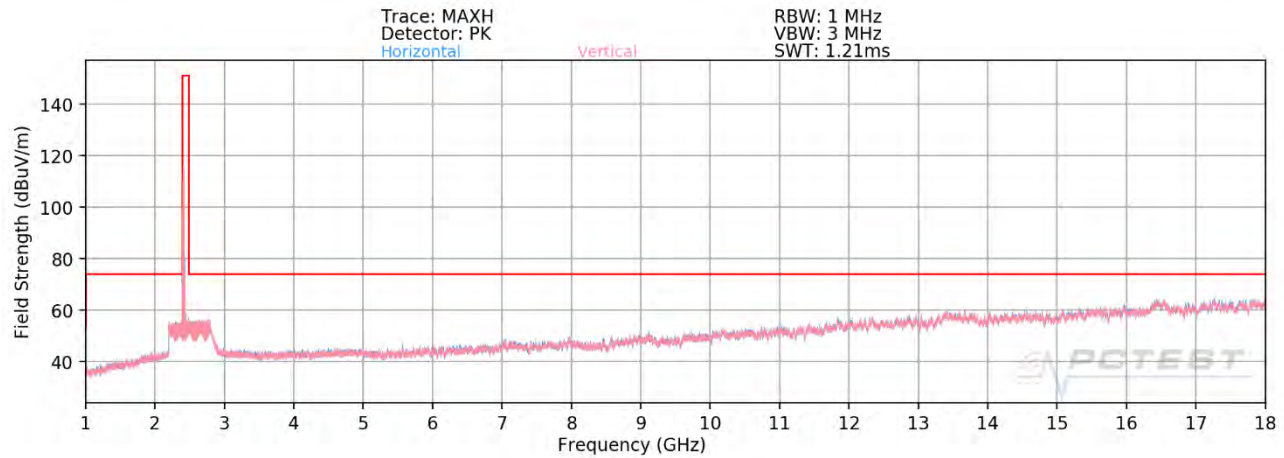
Plot 7-111. Radiated Spurious Plot above 1GHz MIMO/CDD (802.11g – Ch. 1)
