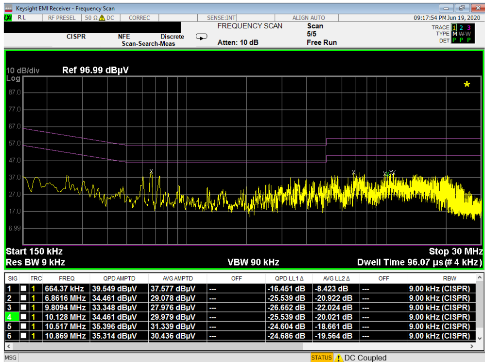
Plot 7-145. Line Conducted Plot with 802.11b (N)
