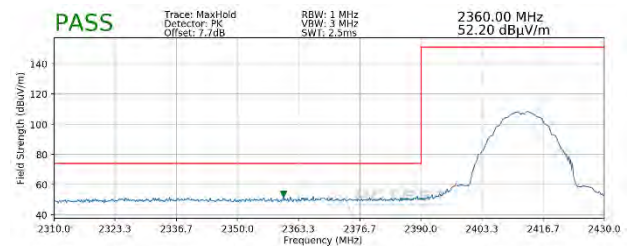
Plot 7-116. Radiated Restricted Lower Band Edge Measurement SISO ANT1 (Peak)
