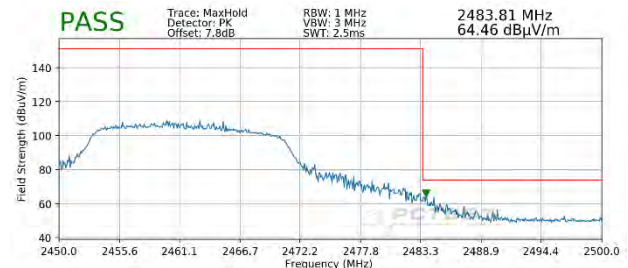
Plot 7-134. Radiated Restricted Upper Band Edge Measurement SISO ANT2 (Peak)
