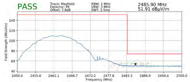
Plot 7-120. Radiated Restricted Upper Band Edge Measurement SISO ANT1 (Peak)
