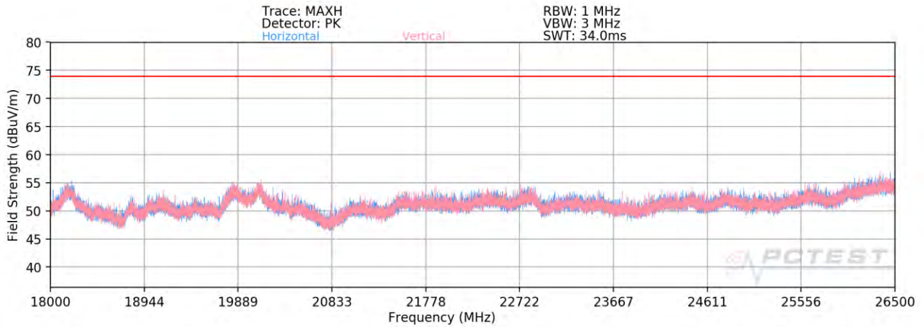
Plot 7-114. Radiated Spurious Plot above 18GHz MIMO/CDD
