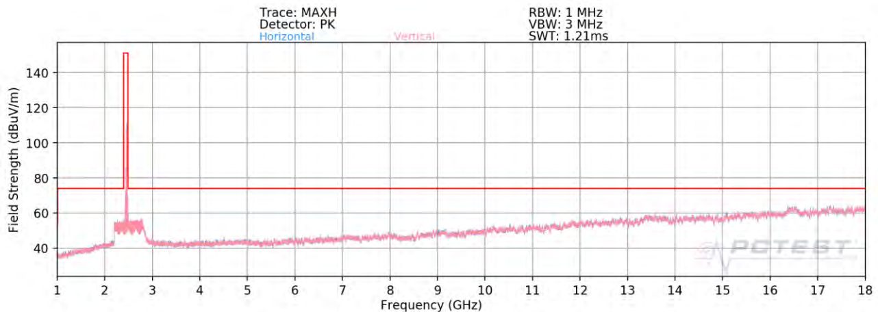
Plot 7-109. Radiated Spurious Plot above 1GHz SISO ANT2 (802.11b – Ch. 11)
