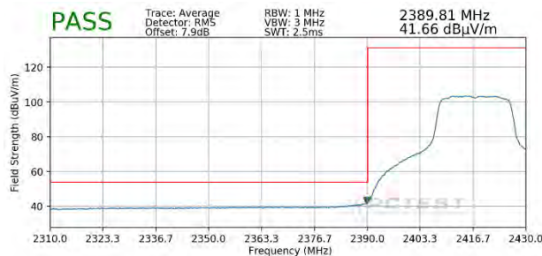
Plot 7-137. Radiated Restricted Lower Band Edge Measurement MIMO (Average)
