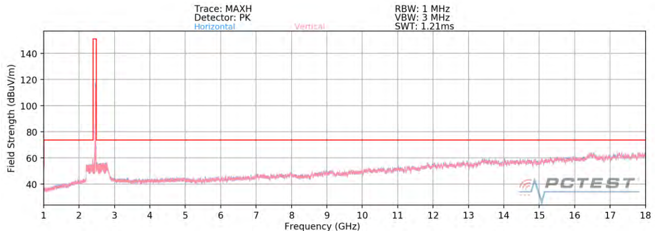
Plot 7-113. Radiated Spurious Plot above 1GHz MIMO/CDD (802.11g – Ch. 11)
