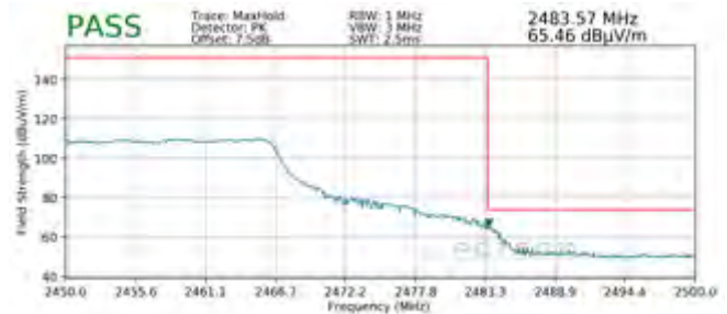
Plot 7-140. Radiated Restricted Upper Band Edge Measurement MIMO (Peak)
