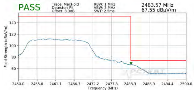
Plot 7-142. Radiated Restricted Upper Band Edge Measurement MIMO (Peak)
