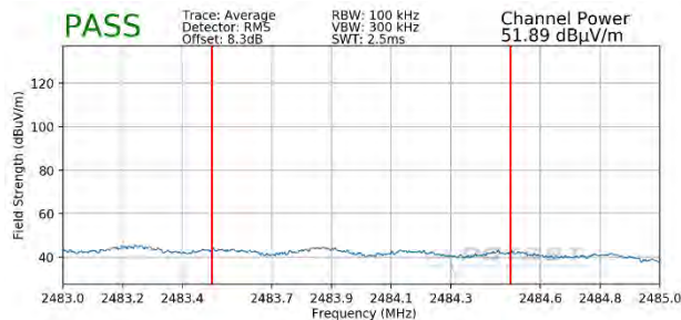
Plot 7-141. Radiated Restricted Upper Band Edge Measurement MIMO (Average)
