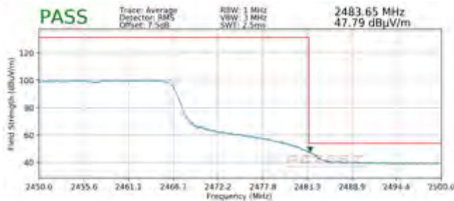
Plot 7-139. Radiated Restricted Upper Band Edge Measurement MIMO (Average)
