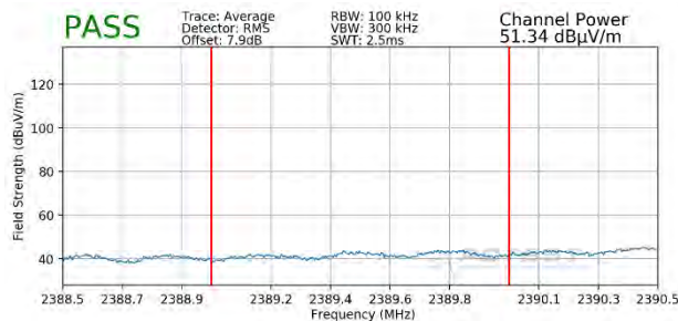
Plot 7-135. Radiated Restricted Lower Band Edge Measurement MIMO (Average)
