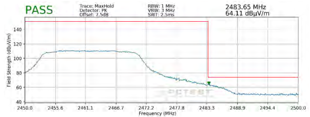
Plot 7-126. Radiated Restricted Upper Band Edge Measurement SISO ANT1 (Peak)
