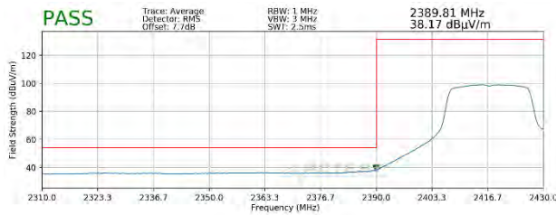
Plot 7-129. Radiated Restricted Lower Band Edge Measurement SISO ANT2 (Average)
