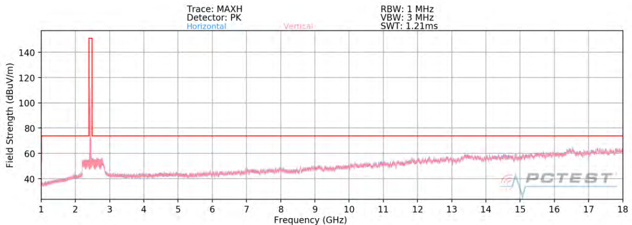
Plot 7-108. Radiated Spurious Plot above 1GHz SISO ANT2 (802.11b – Ch. 6)
