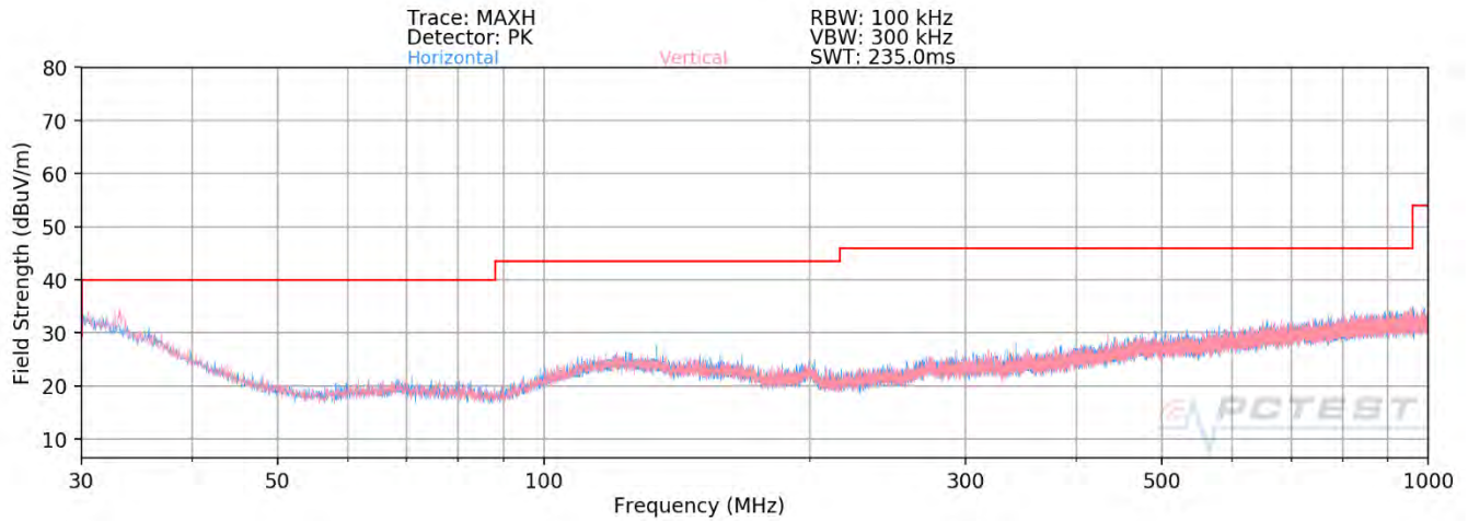
Plot 7-143. Radiated Spurious Plot below 1GHz SISO ANT1
