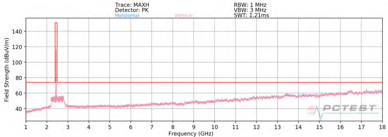
Plot 7-112. Radiated Spurious Plot above 1GHz MIMO/CDD (802.11g – Ch. 6)
