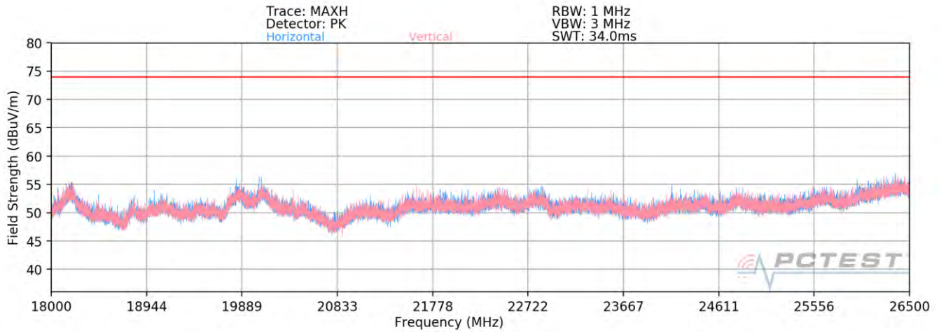
Plot 7-110. Radiated Spurious Plot above 18GHz SISO ANT2
