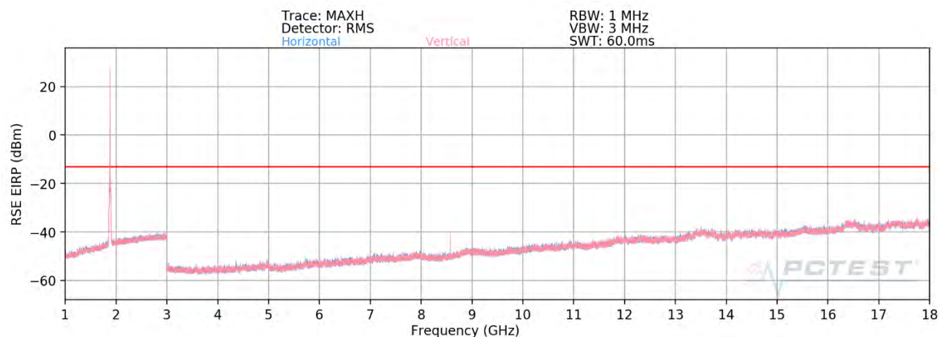
Plot 7-34. Ant 1-n261 Radiated Spurious Plot (1CC QPSK Mid Channel H Beam – EN-DC Anchor Band 2)
