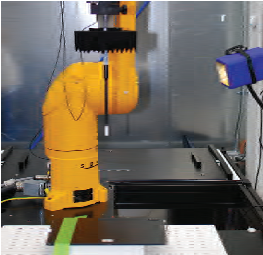
Test Setup Photo 6 – Power Density Setup (Figure 7-2)
