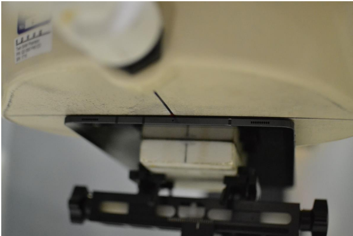
SAR Test Setup Photo 7 – Back Side at 0 mm for WIFI MIMO
