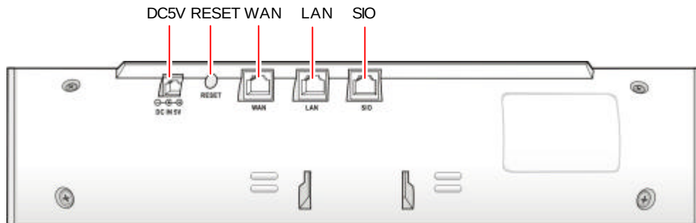
Figure 1.2 Rear Panel of SMT-R2000
