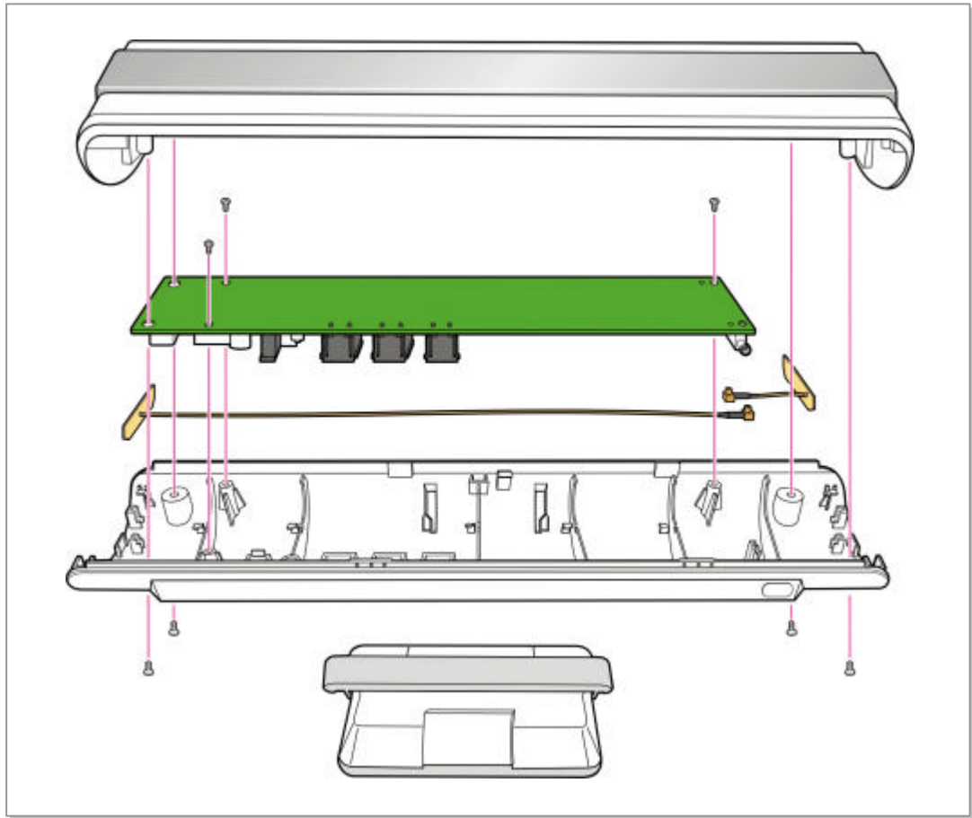
Figure 2.9 SMT-R2000 Disassembly Diagram
