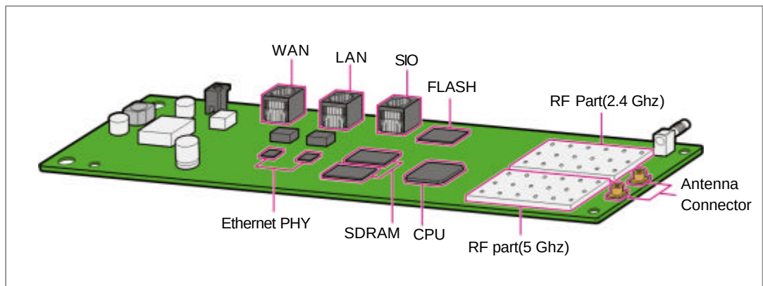
Figure 2.1 Configuration of SMT-R2000 Main Board
