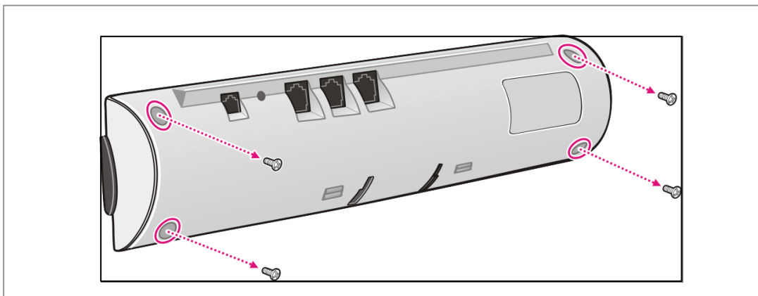
Figure 2.3 Removing Case Screws
