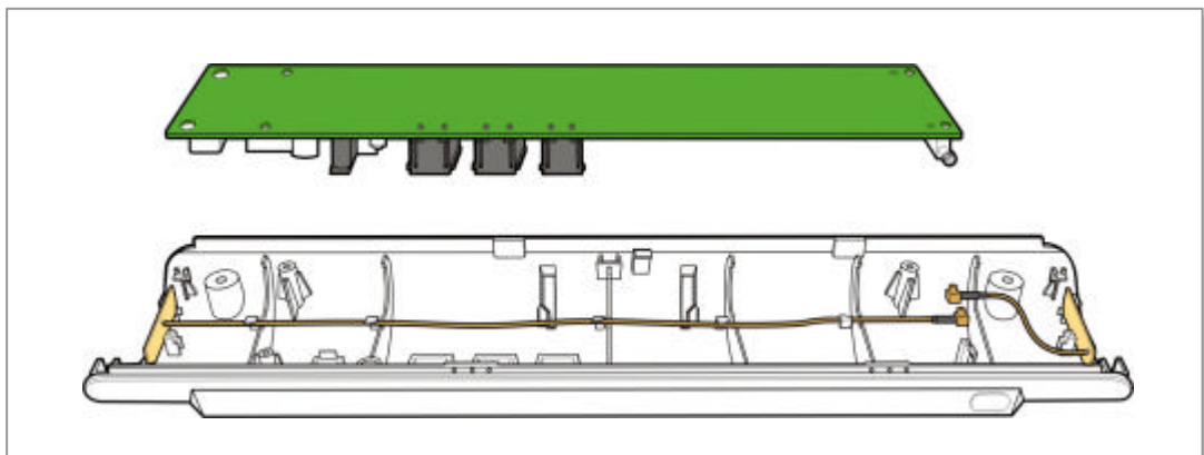
Figure 2.6 Separating the Main Board and Bottom Case
