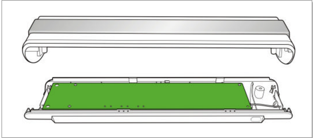
Figure 2.4 Separating the Case
