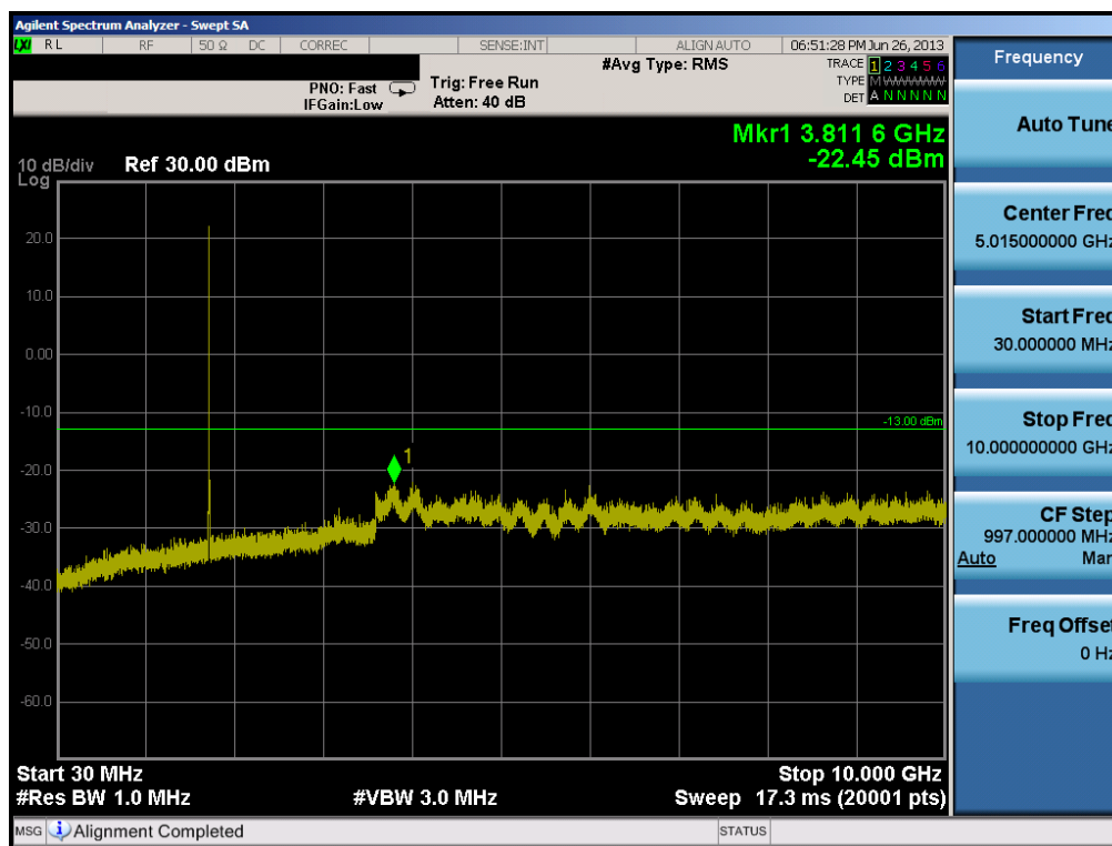
Plot 6-31. Conducted Spurious Plot (AWS WCDMA Mode – Ch. 1412)
