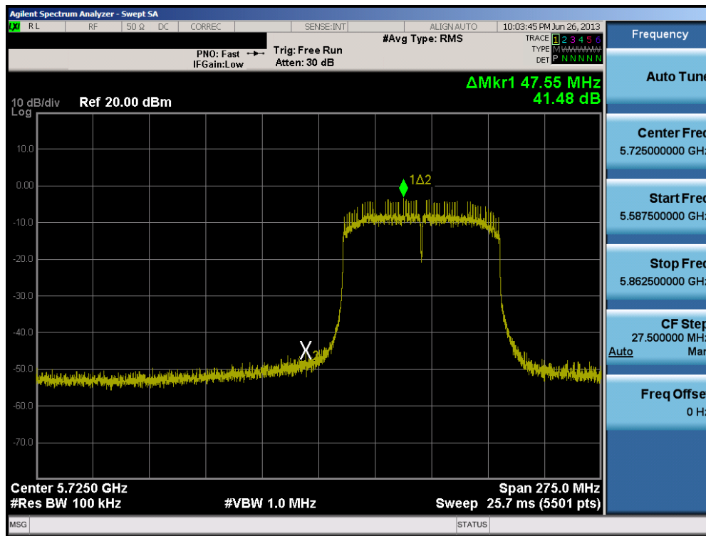
Plot 6-49. Band Edge Plot (80MHz BW 802.11ac (5.8GHz) – Ch. 155)
