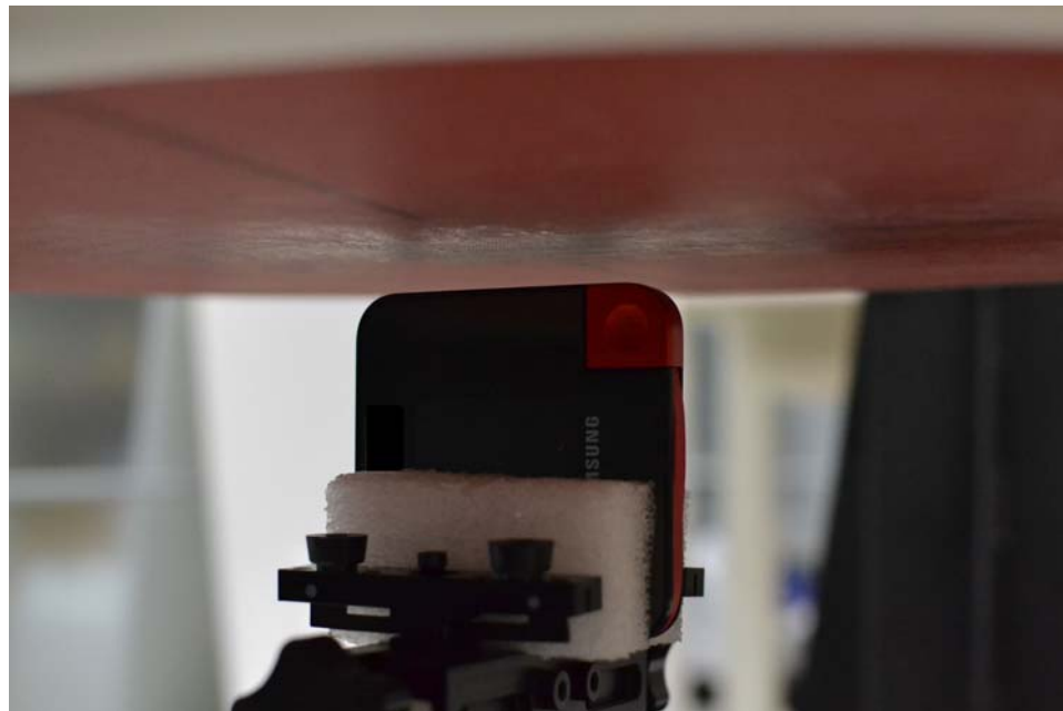
SAR Test Setup Photo 4 - Right Edge at 10 mm
