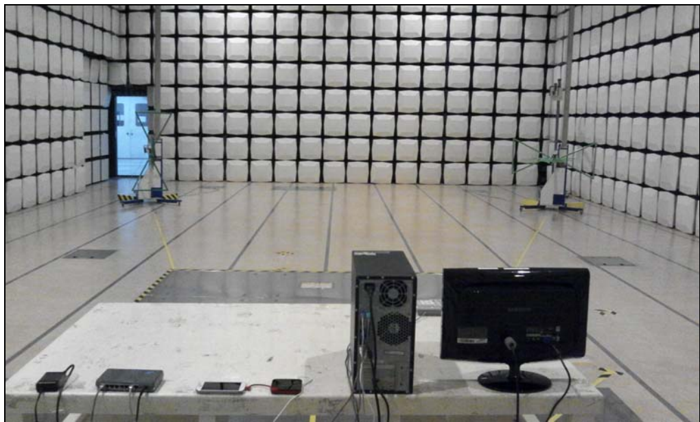
[ Radiated Disturbance for Below 1 GHz – Rear ]
