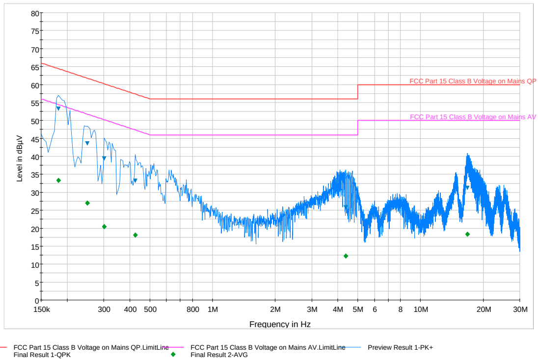
Plot 7-1. Line Conducted Plot (L1)
