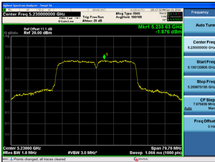
802.11n_HT40 UNII 1 BAND PSD CH 46
