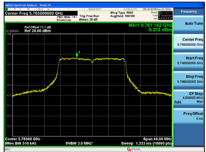
802.11a UNII 3 BAND PSD CH 153
