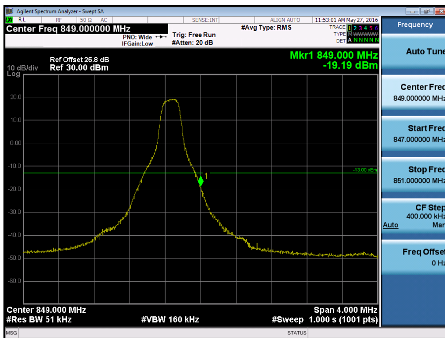
BAND 5. Upper Band Edge Plot (5M BW Ch.20625 QPSK_RB1_Offset 24)
