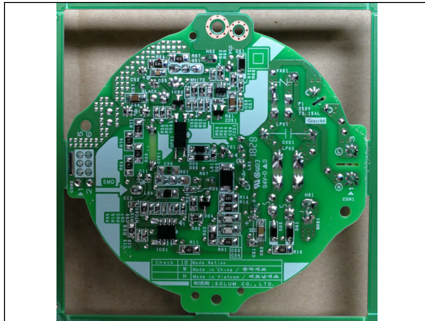
Bottom view of Sub PCB5
