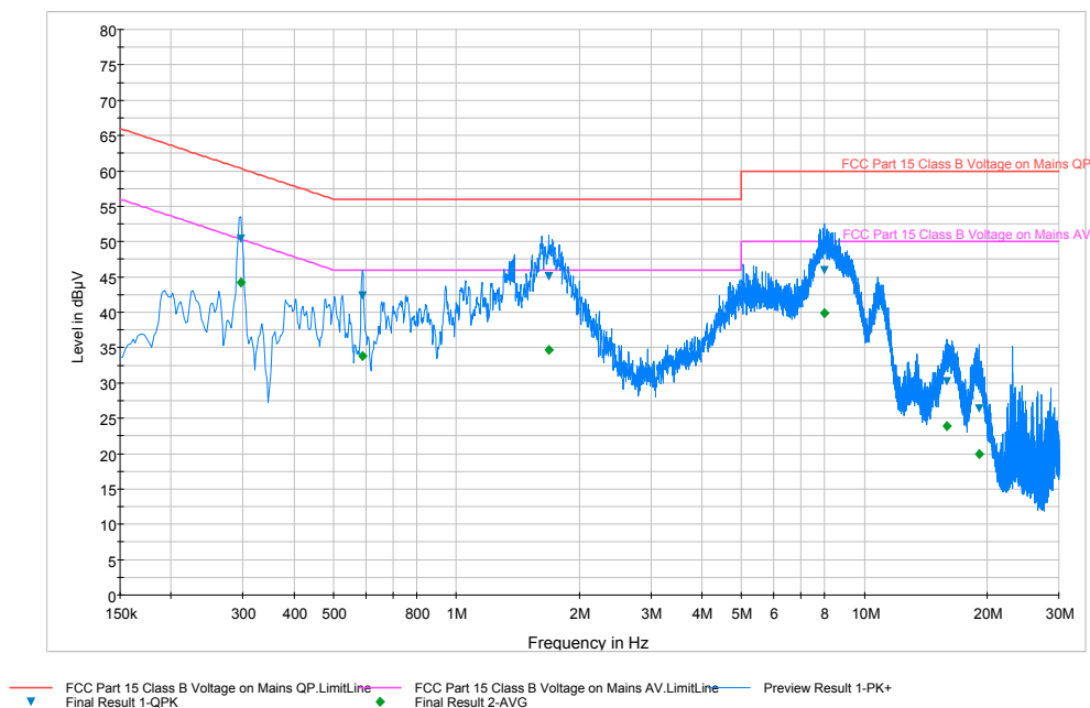
Plot 6-20. Line Conducted Plot with Bluetooth LE (L1)
