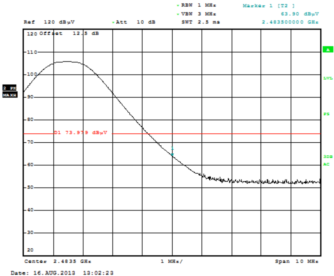
Plot 6-19. Radiated Restricted Upper Band Edge Measurement (Peak)
