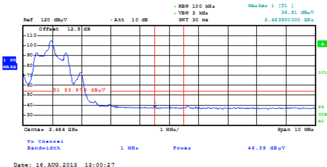
Plot 6-18. Radiated Restricted Upper Band Edge Measurement (Average)
