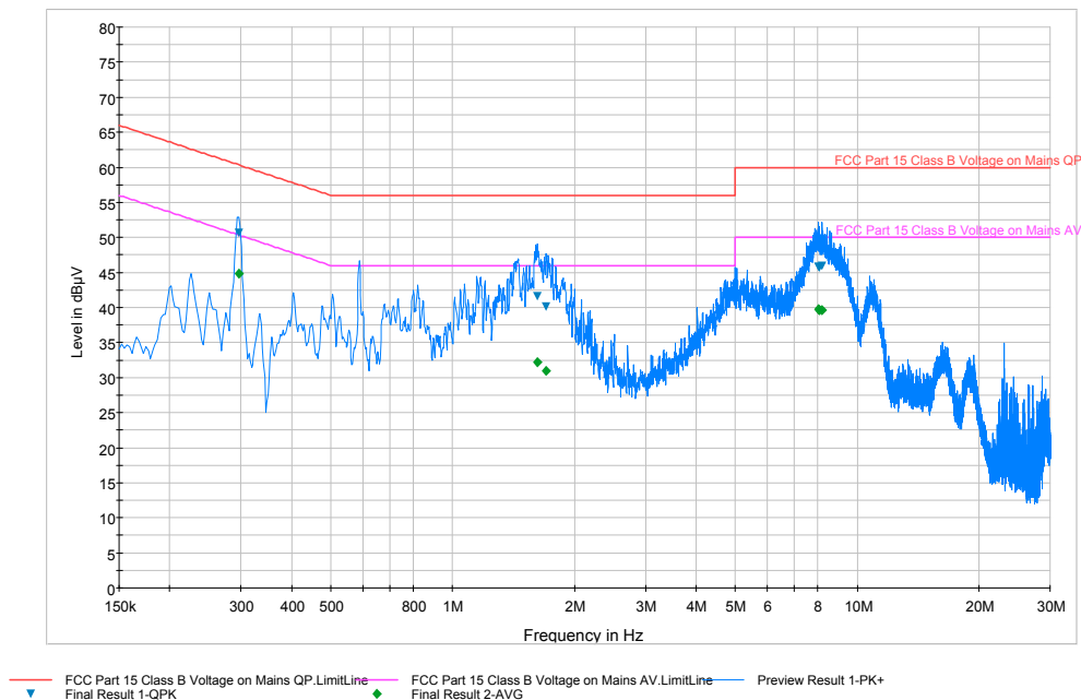
Plot 6-21. Line Conducted Plot with Bluetooth LE (N)
