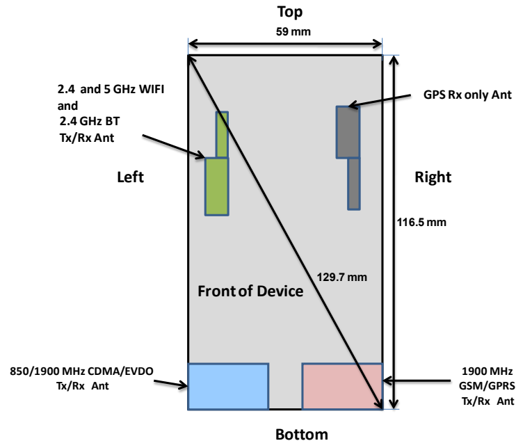
Figure 1-1 DUT Antenna Locations
