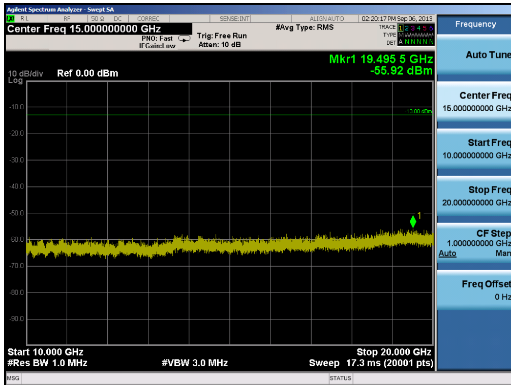
Plot 6-19. Conducted Spurious Plot (PCS CDMA Mode – Ch. 600)
