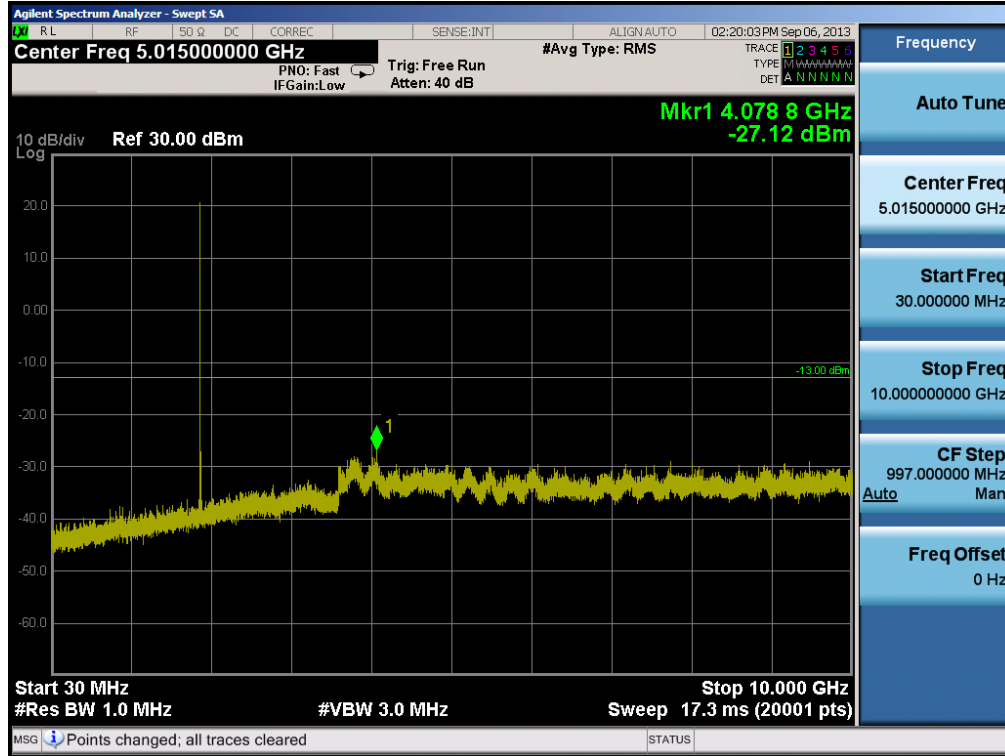
Plot 6-18. Conducted Spurious Plot (PCS CDMA Mode – Ch. 600)
