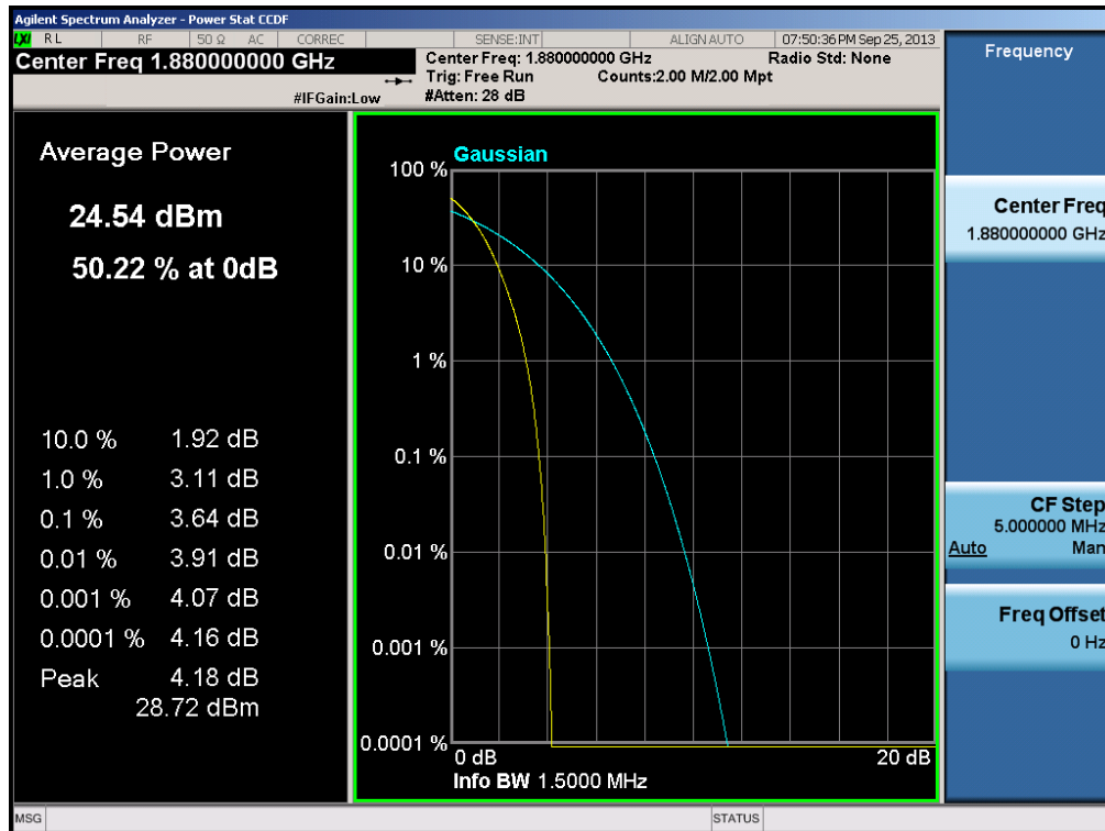
Plot 6-33. Peak-Average Ratio Plot (PCS CDMA Mode – Ch. 600)
