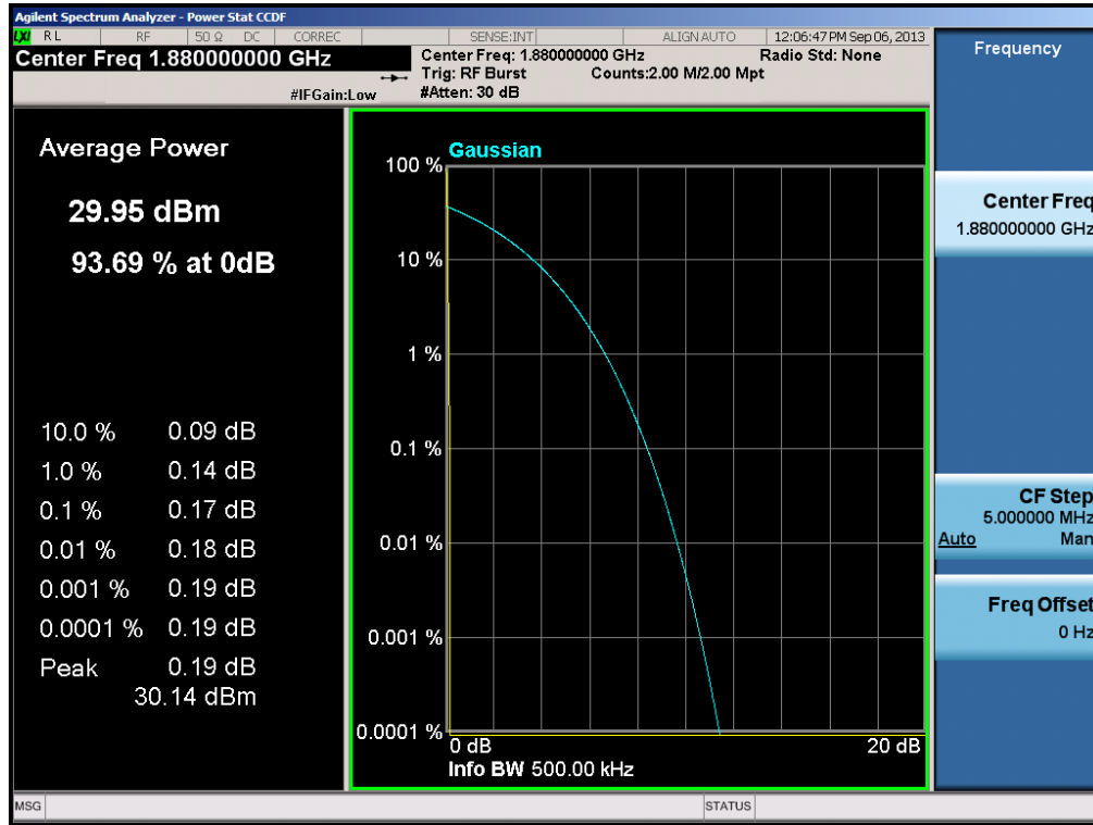
Plot 6-32. Peak-Average Ratio Plot (PCS GSM Mode – Ch. 661)
