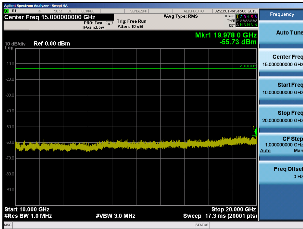
Plot 6-17. Conducted Spurious Plot (PCS CDMA Mode – Ch. 25)
