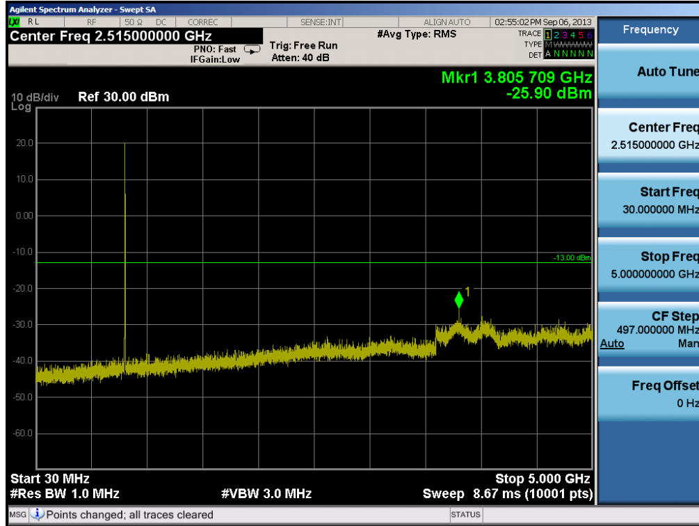
Plot 6-10. Conducted Spurious Plot (Cellular CDMA Mode – Ch. 1013)
