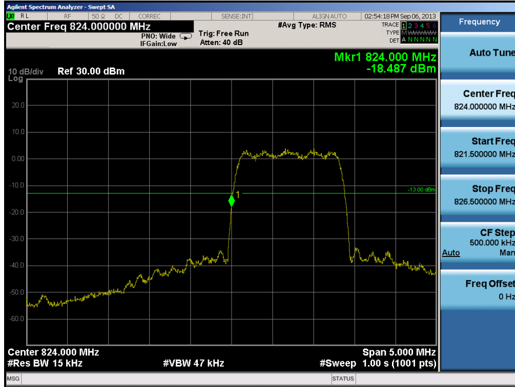
Plot 6-24. Band Edge Plot (Cellular CDMA Mode – Ch. 1013)
