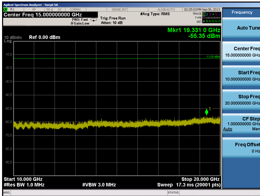
Plot 6-21. Conducted Spurious Plot (PCS CDMA Mode – Ch. 1175)
