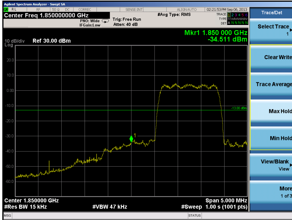
Plot 6-28. Band Edge Plot (PCS CDMA Mode – Ch. 25)
