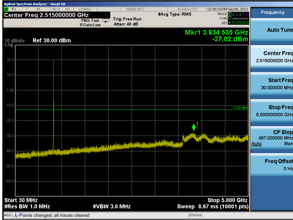
Plot 6-14. Conducted Spurious Plot (Cellular CDMA Mode – Ch. 777)
