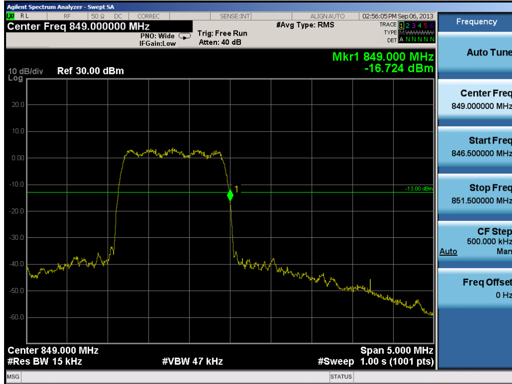
Plot 6-26. Band Edge Plot (Cellular CDMA Mode – Ch. 777)
