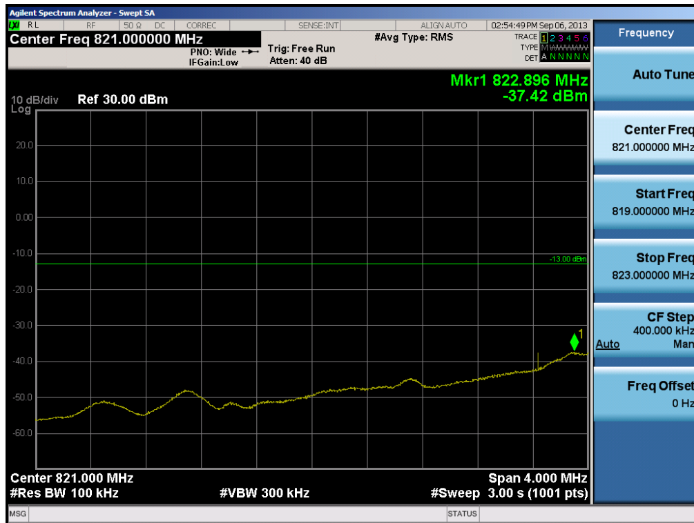
Plot 6-25. 4MHz Span Plot (Cellular CDMA Mode – Ch. 1013)
