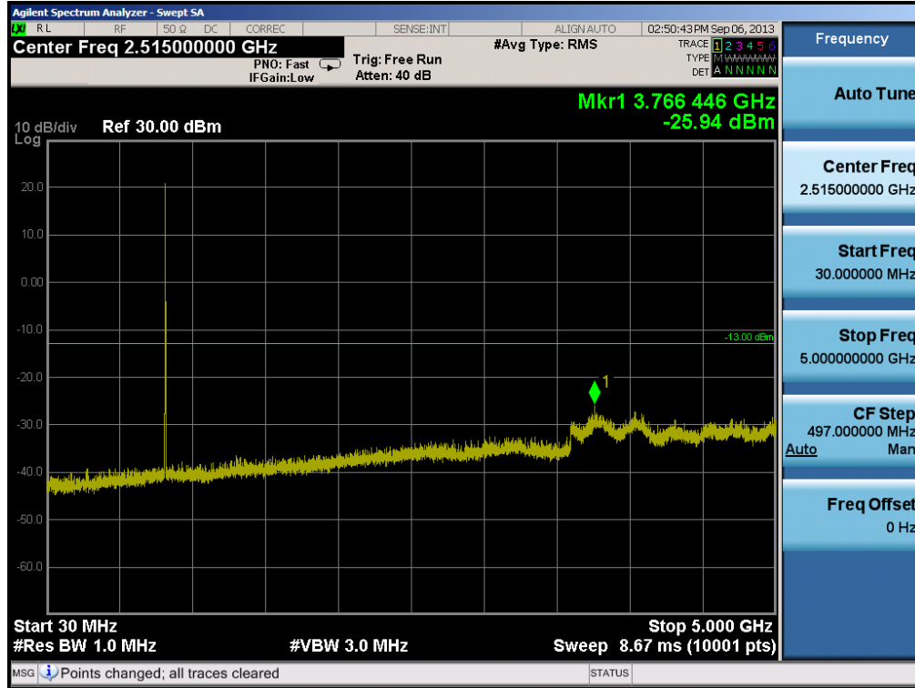
Plot 6-12. Conducted Spurious Plot (Cellular CDMA Mode – Ch. 384)
