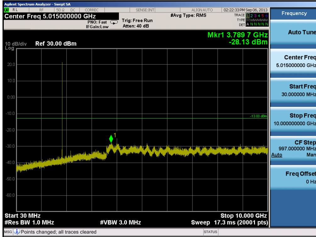
Plot 6-16. Conducted Spurious Plot (PCS CDMA Mode – Ch. 25)
