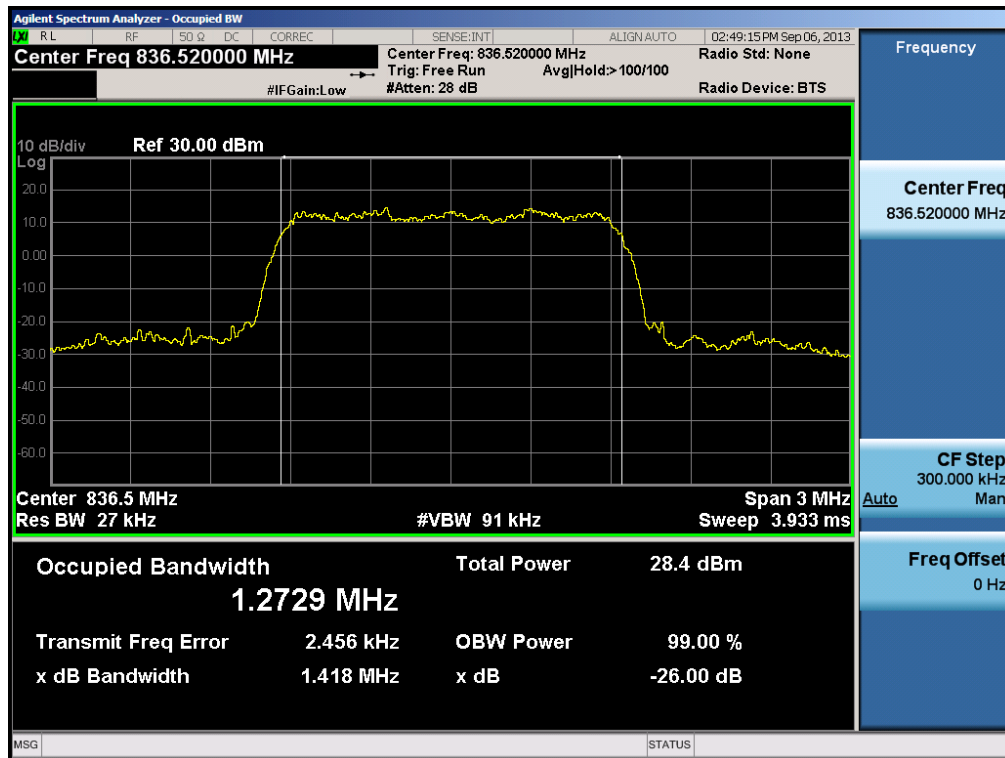
Plot 6-2. Occupied Bandwidth Plot (Cellular CDMA Mode – Ch. 384)
