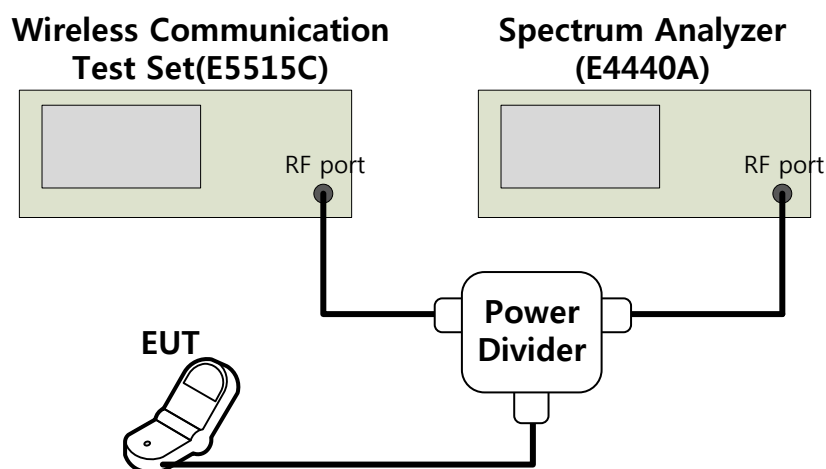
Figure 6-5. Test Instruments & Measurement Setup
