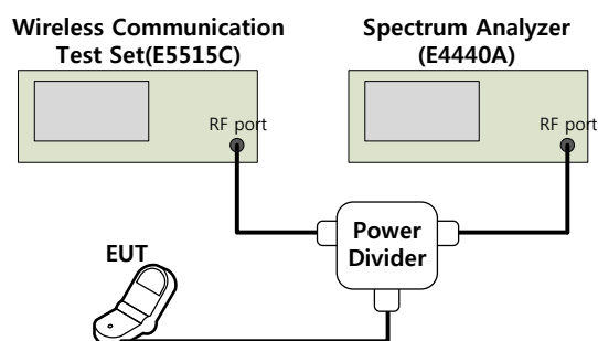
Figure 6-1. Test Instruments & Measurement Setup
