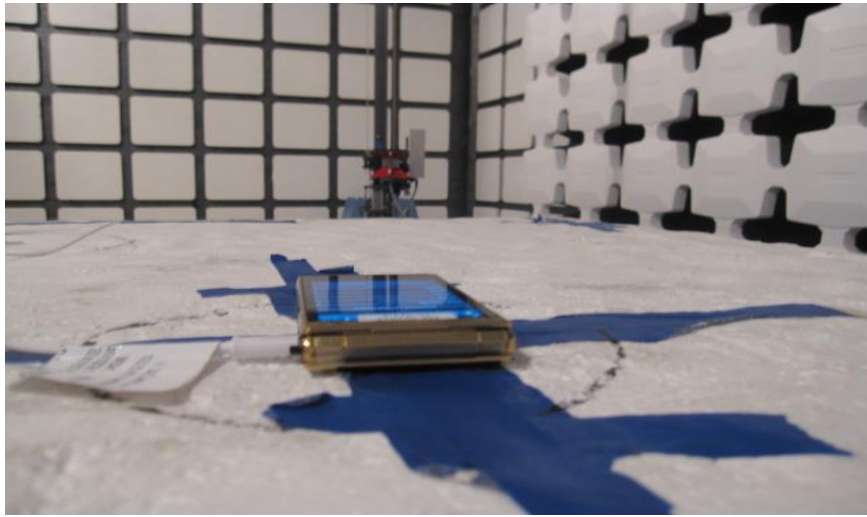
X-AXIS FRONT PHOTO
