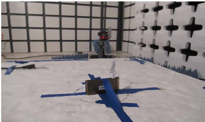
Y-AXIS FRONT PHOTO
