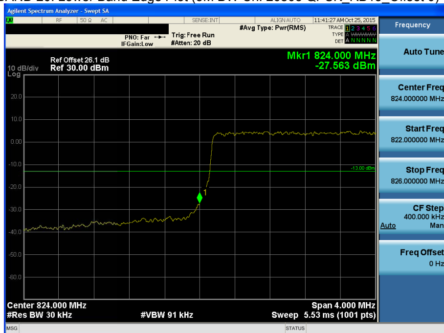
BAND 26. Lower Band Edge Plot (3M BW Ch. 26805 QPSK RB15 Offset 0) -2
