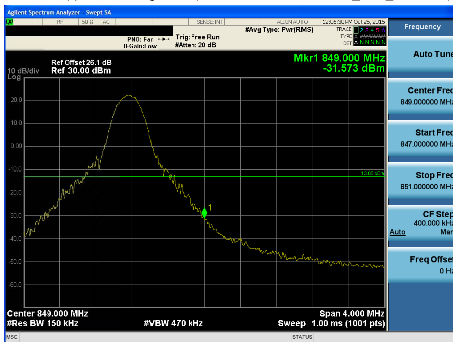
BAND 26. Upper Band Edge Plot (15M BW Ch.26965 QPSK_RB1_Offset 74) -1
