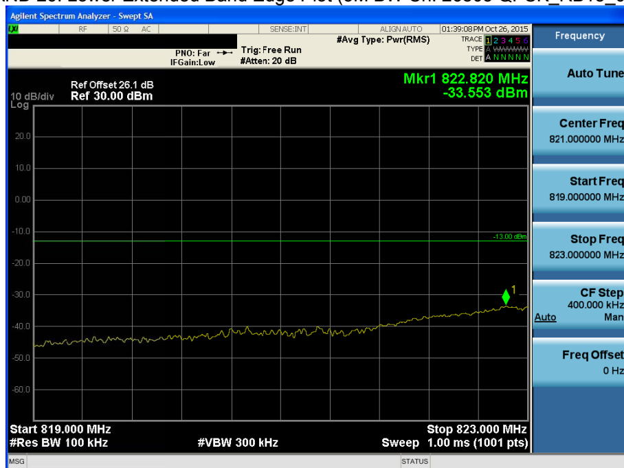
BAND 26. Lower Extended Band Edge Plot (3M BW Ch. 26805 QPSK RB15 0)-3
