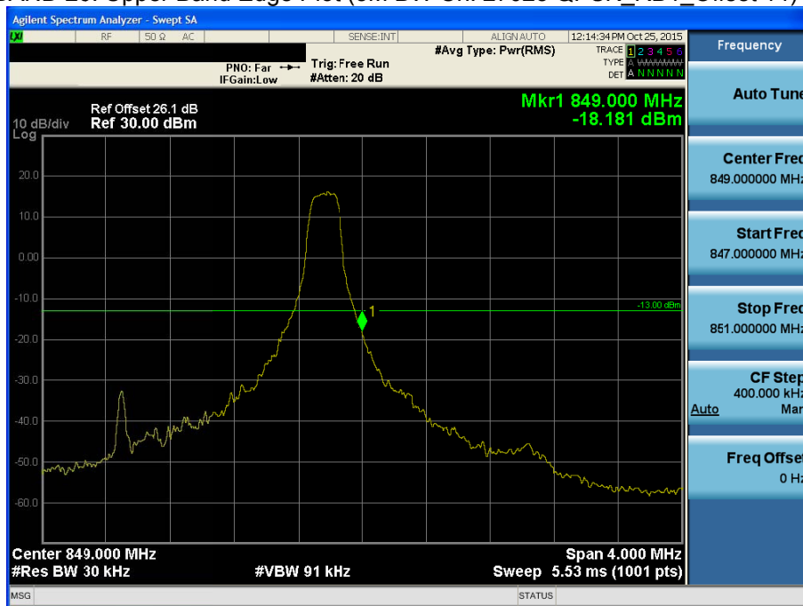
BAND 26. Upper Band Edge Plot (3M BW Ch. 27025 QPSK_RB1_Offset 14) -1
