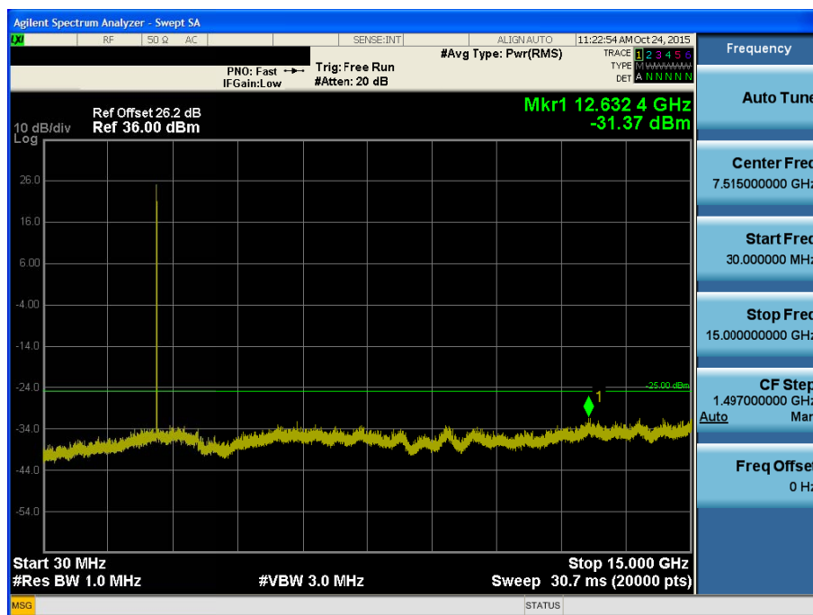
BAND 41. Conducted Spurious Plot 1 (5 MHz Ch.41215 QPSK RB 1, Offset 0)
