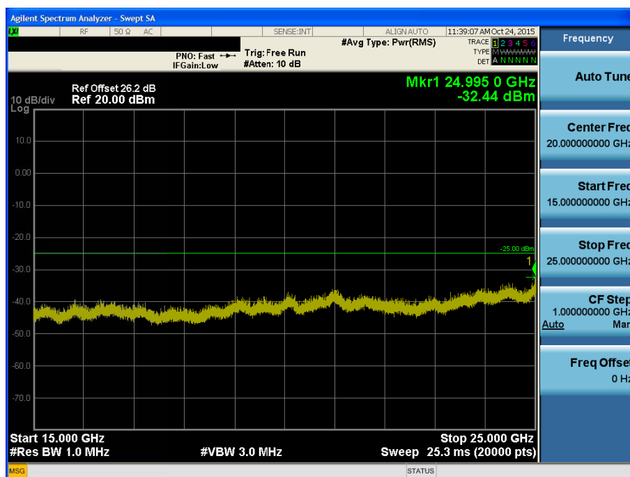
BAND 41. Conducted Spurious Plot 2 (5 MHz Ch. 41215 QPSK RB 1, Offset 0)
