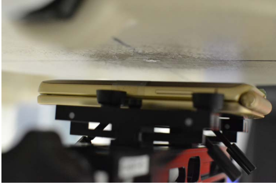
SAR Test Setup Photo 9 – Back Side at 15 mm
