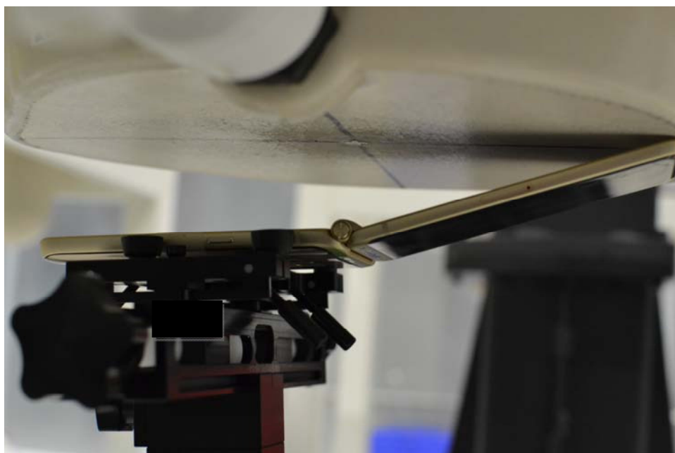
SAR Test Setup Photo 6 – Mouth-Jaw Replacing Left Cheek
