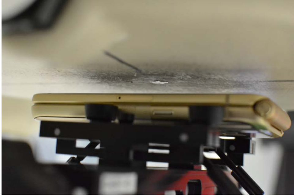
SAR Test Setup Photo 11 – Front Side at 10 mm
