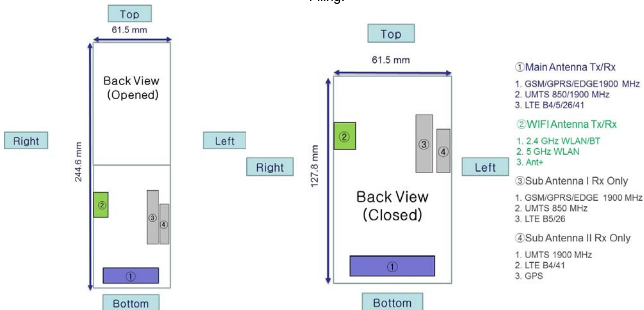
Figure F-1 DUT Antenna Locations
