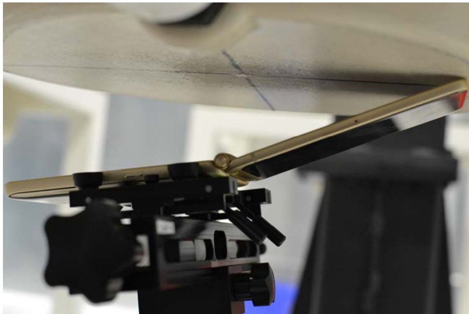
SAR Test Setup Photo 8 – Mouth-Jaw Replacing Left Tilt
