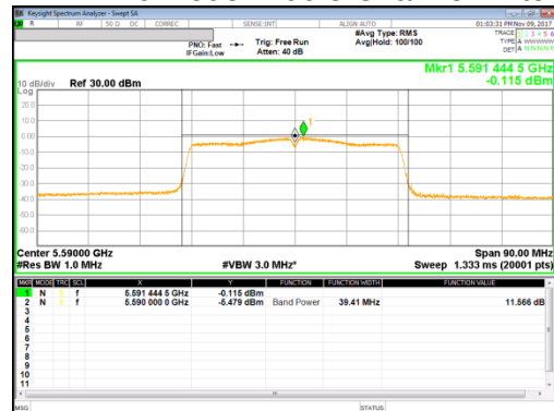
11n HT40 Mode High Channel Antenna 1
