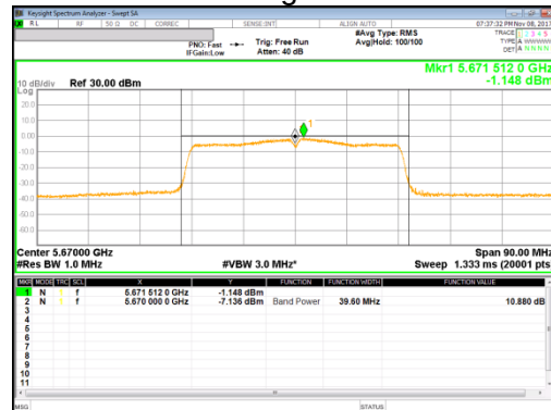
11n HT40 Mode Straddle Channel Antenna 2
