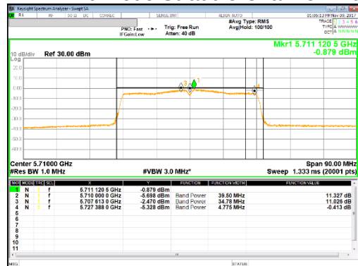
11n HT40 Mode Straddle Channel Antenna 1
