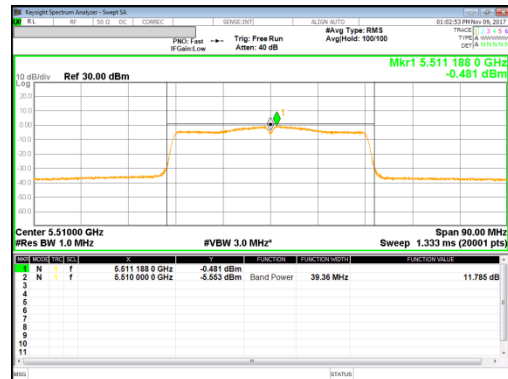
11n HT40 Mode Middle Channel Antenna 1
