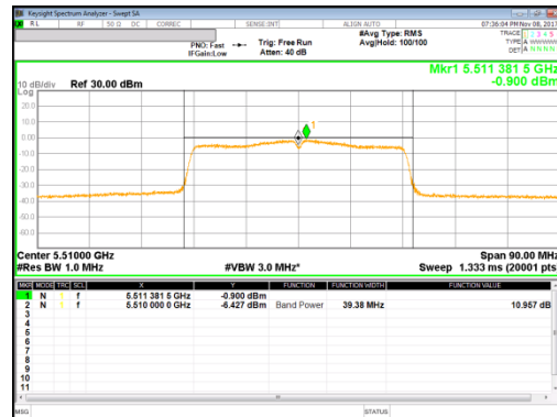
11n HT40 Mode Middle Channel Antenna 2
