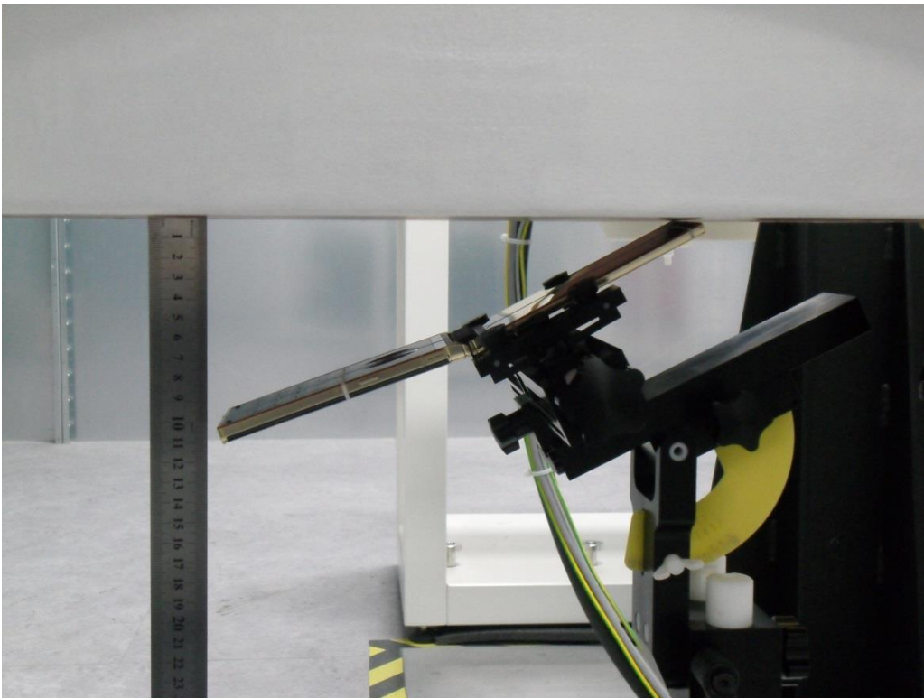
Tilt (15°) condition at flat phantom
