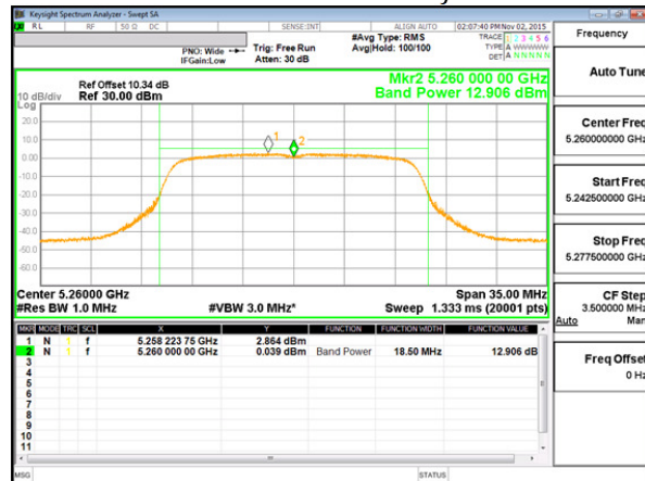
11a Mode Middle Channel Primary
