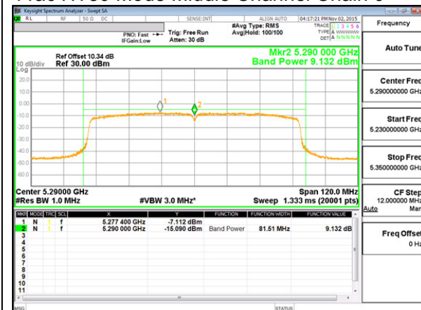
11ac HT80 Mode Middle Channel Chain 0
