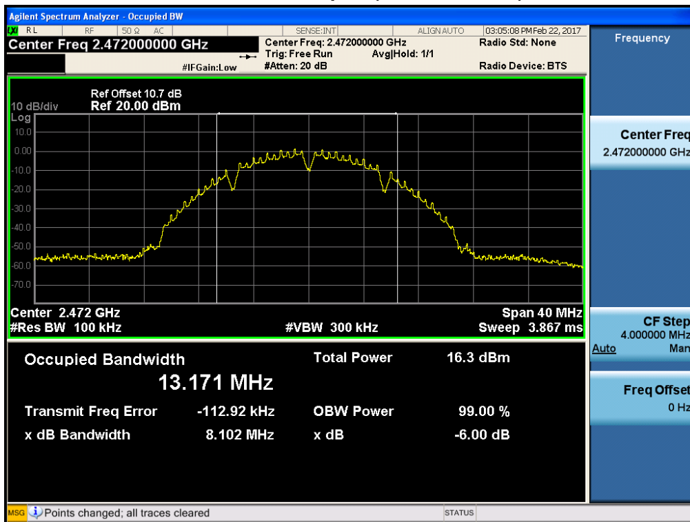
6dB Bandwidth plot (802.11b-CH 13)
