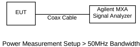
Figure 9-4 Power Measurement Setup
