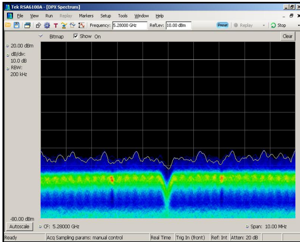
Figure 5-3. Real-Time Spectrum Display, WLAN Traffic (Streaming Video)
