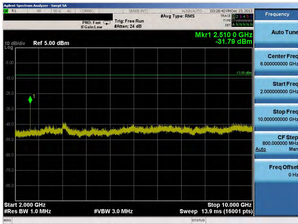
Plot 6-14. Conducted Spurious Plot (Cellular GSM Mode – Ch. 190)
