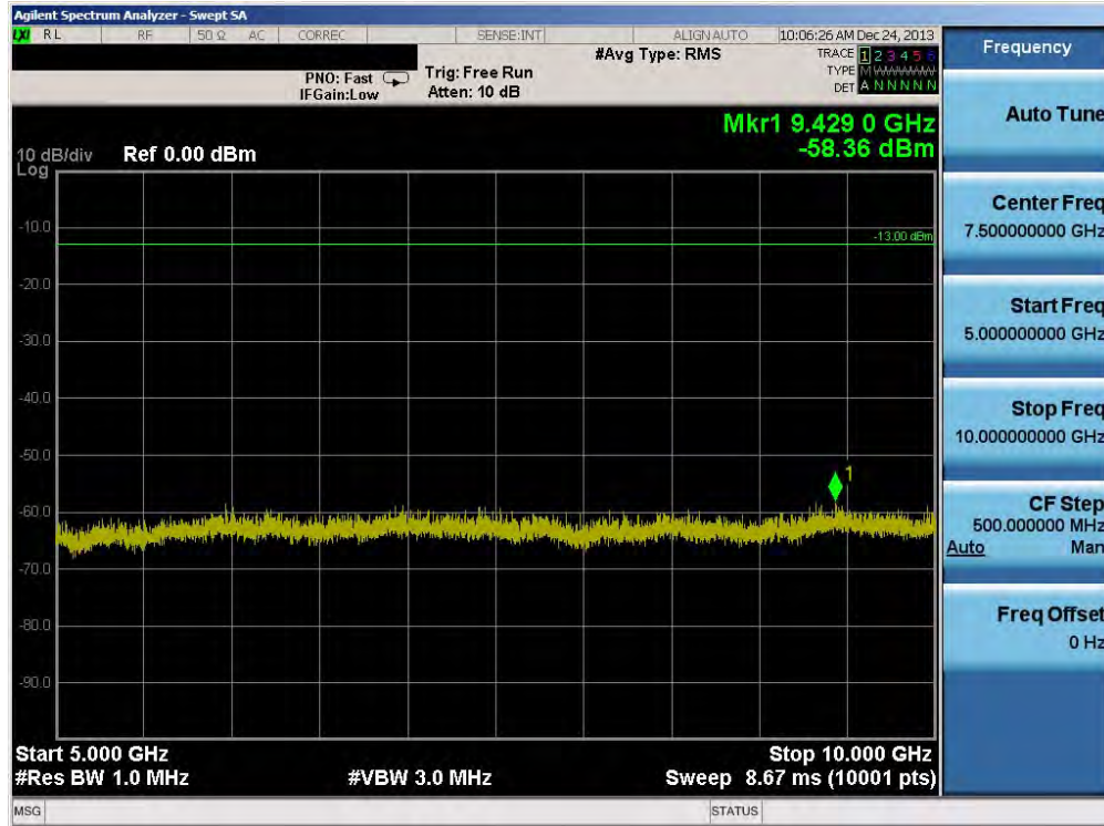
Plot 6-29. Conducted Spurious Plot (Cellular CDMA Mode – Ch. 777)
