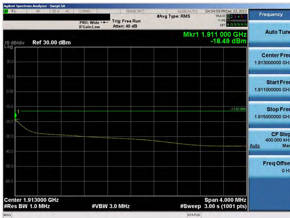
Plot 6-65. 4MHz Span Plot (PCS WCDMA Mode – Ch. 9538)
