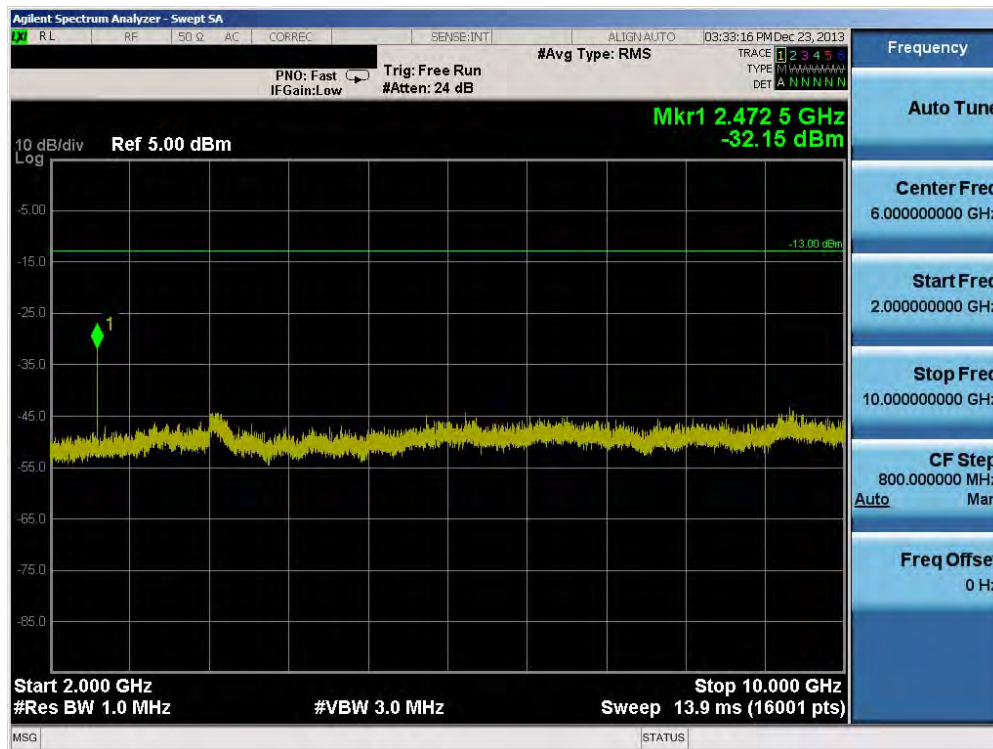
Plot 6-11. Conducted Spurious Plot (Cellular GSM Mode – Ch. 128)
