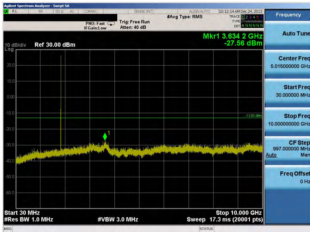
Plot 6-30. Conducted Spurious Plot (PCS CDMA Mode – Ch. 25)
