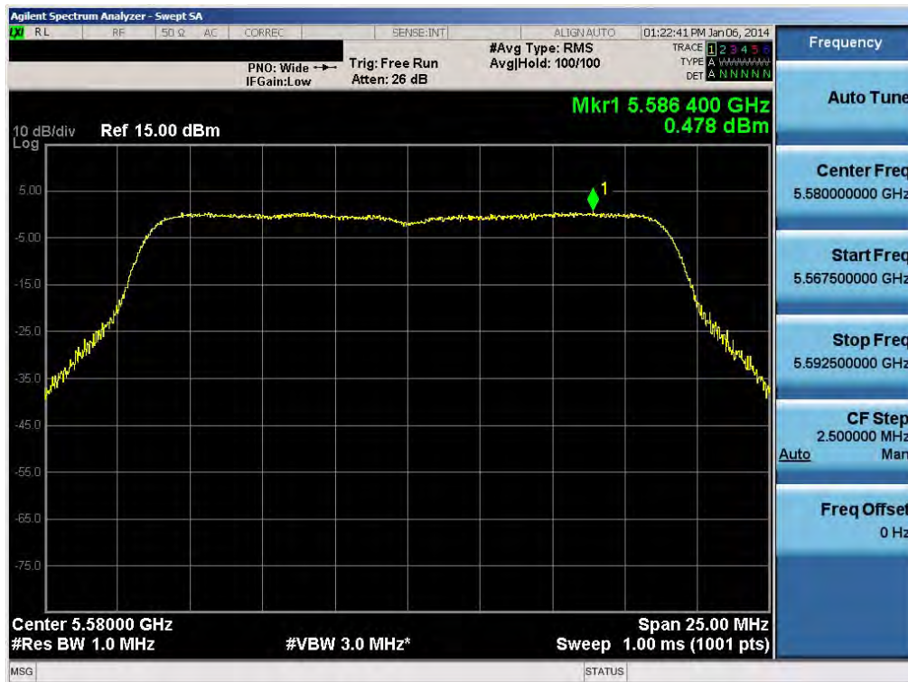
Plot 6-57. Peak Power Spectral Density Plot (20MHz BW 802.11n (UNII Band 2C) – Ch. 116)
