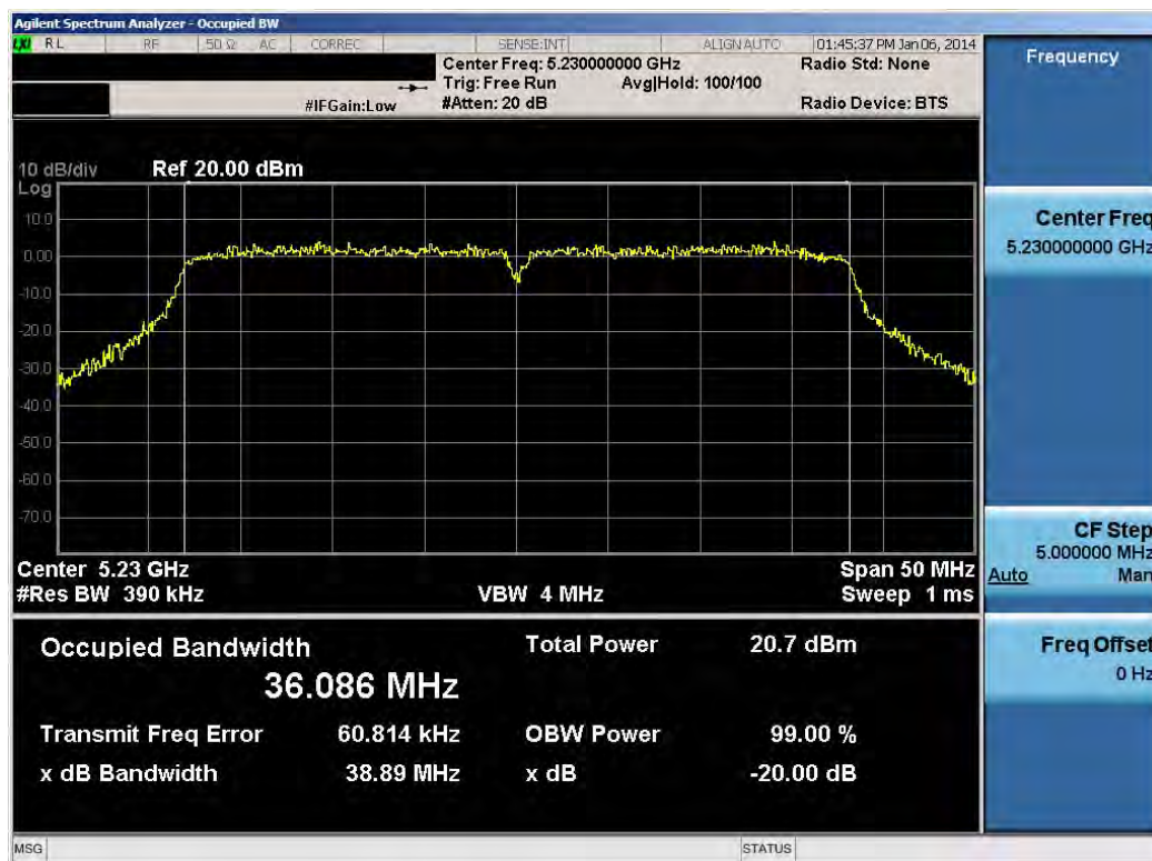
Plot 6-30. 20dB Bandwidth Plot (40MHz BW 802.11ac (UNII Band 1) – Ch. 46)
