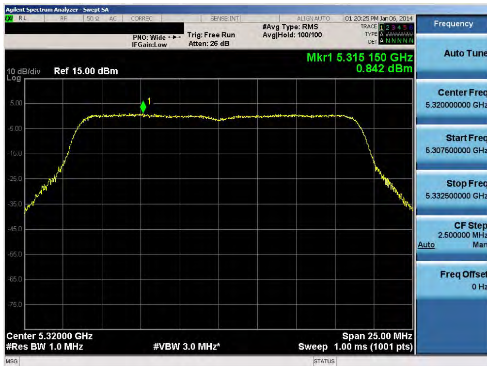
Plot 6-49. Peak Power Spectral Density Plot (20MHz BW 802.11n (UNII Band 2A) – Ch. 64)
