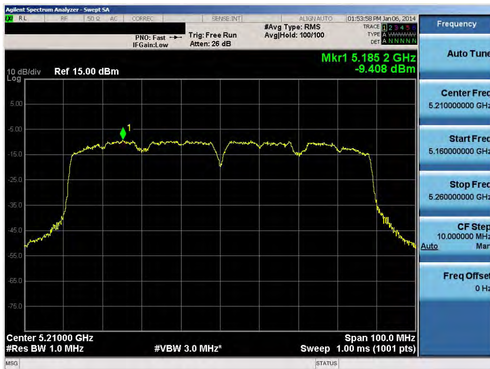
Plot 6-43. Peak Power Spectral Density Plot (80MHz BW 802.11ac (UNII Band 1) – Ch. 42)
