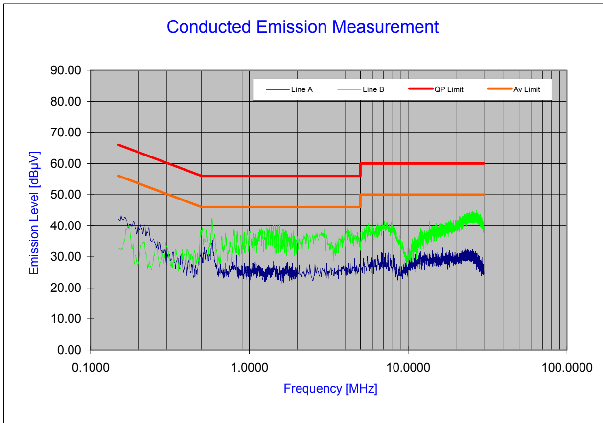
Plot 6-66. Line Conducted Plot with 802.11b
