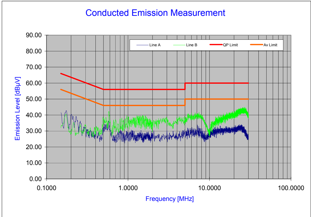
Plot 6-65. Line Conducted Plot with 802.11a
