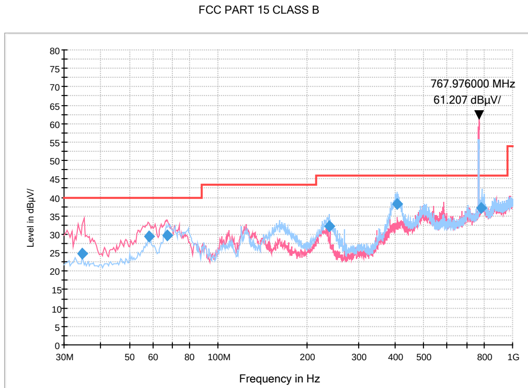
Figure 5: Radiated Emission, Receiver mode (LTE B14 High CH Idle)
