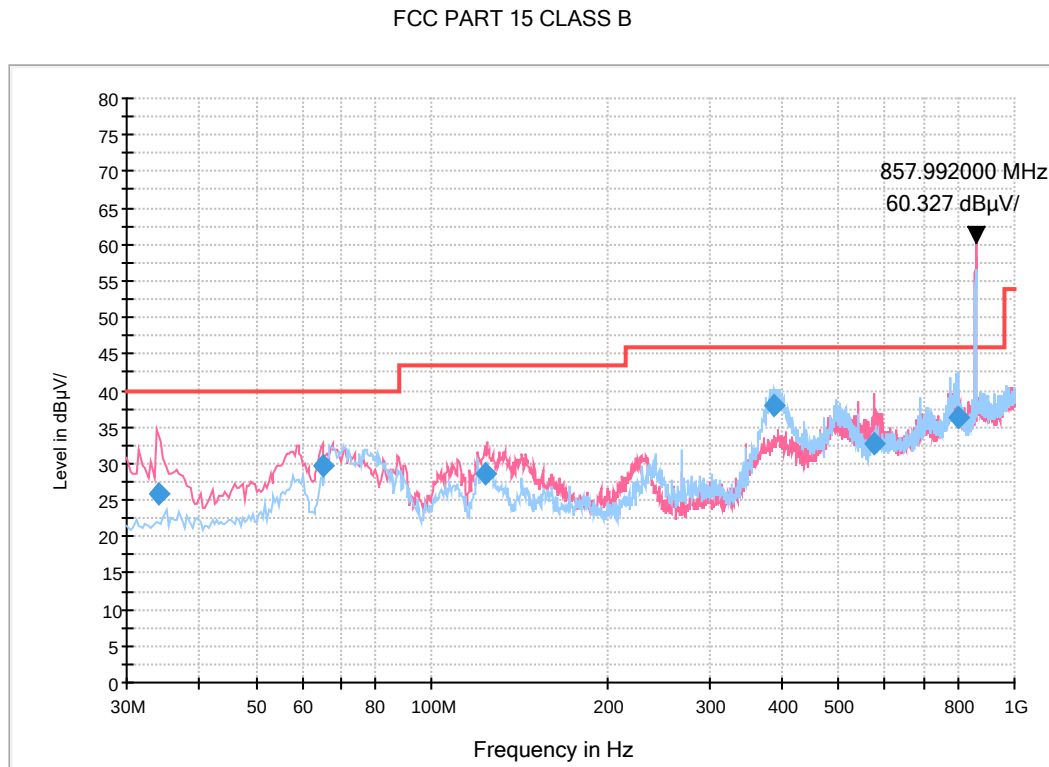
Figure 3: Radiated Emission, Receiver mode (LTE B26+B5 Low CH Idle)
