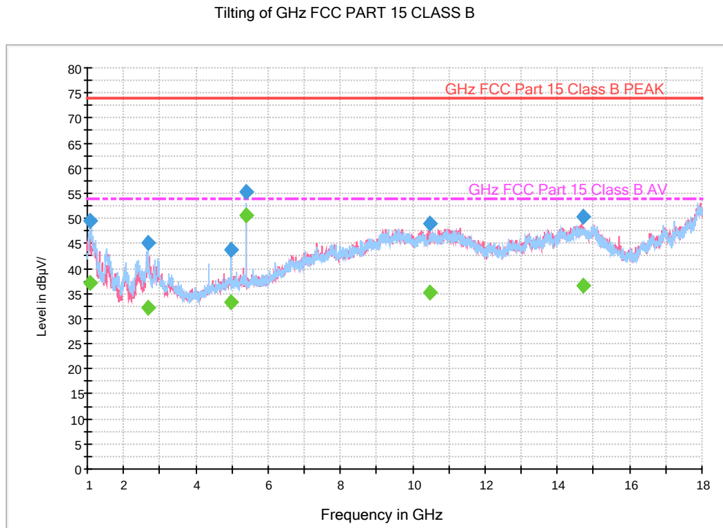
Figure 6: Radiated Emission, Receiver mode (LTE B14 High CH Idle)
