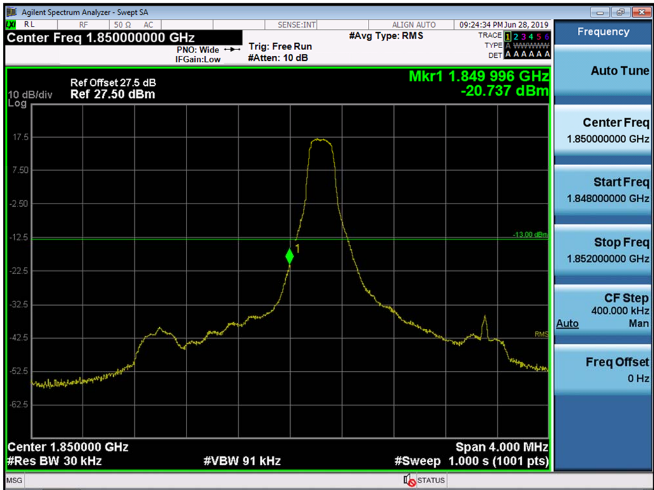
BAND 25/2. Lower Band Edge Plot (3M BW Ch.26055 QPSK_RB1_Offset 0) -1
