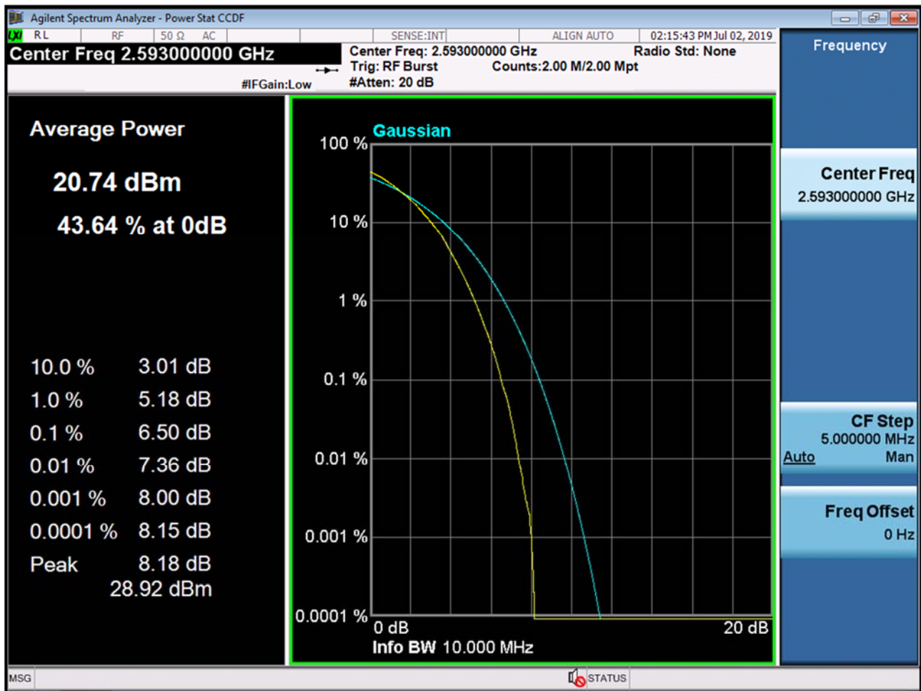
BAND 41. PAR Plot (10M BW_Ch.40620_64QAM_RB50_0)
