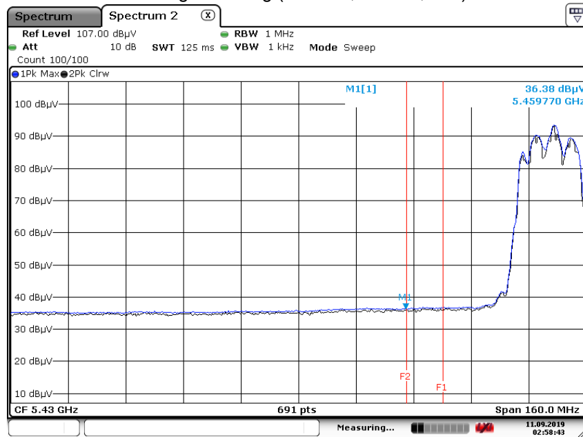
Average Reading (802.11a, Ch.100, Y-V)
