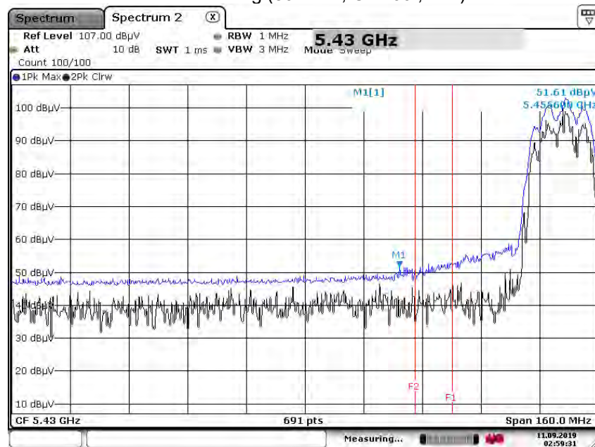
Peak Reading (802.11a, Ch.100, Y-V)
