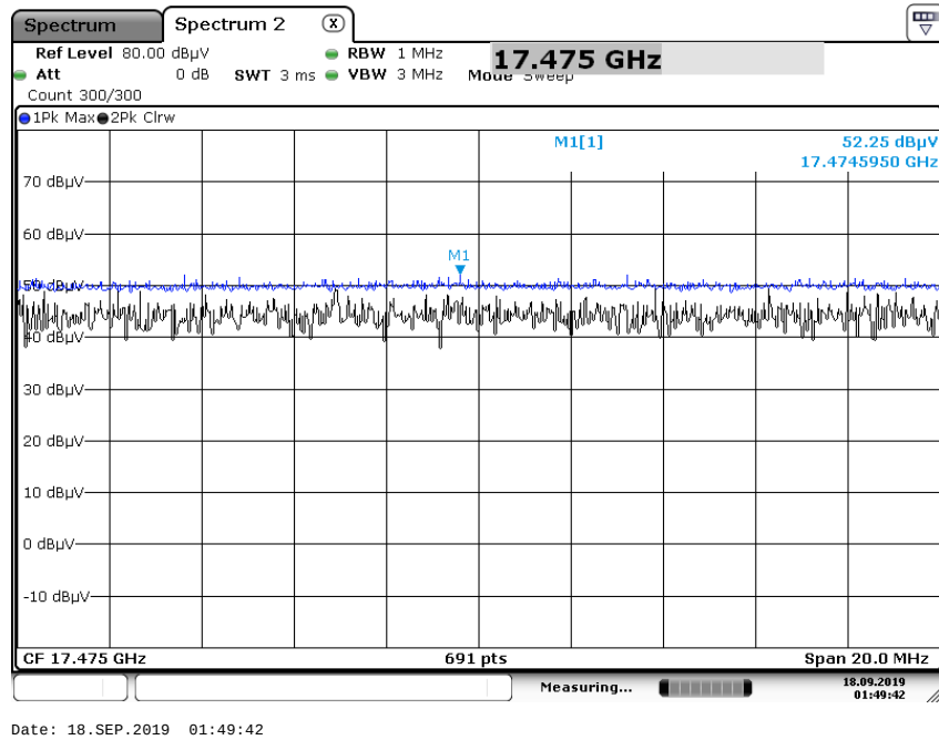
Peak Reading [DBS Mode 2.4 GHz & 5GHz_802.11 a & 802.11b, 6 Mbps & 1Mbps, 165 Ch & 11 Ch]
