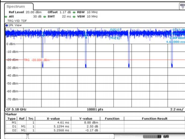
802.11ax_HE20 / 52T
