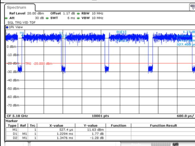
802.11ax_HE20 / 106T
