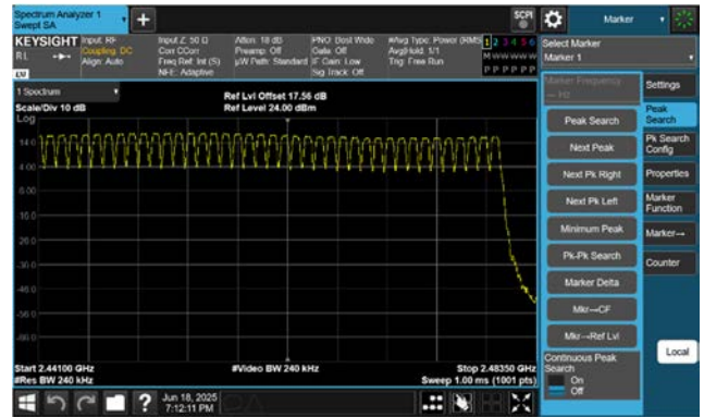
8DPSK (2.441 GHz - 2.483.5 GHz)
