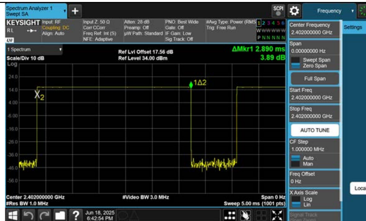
8DPSK : Dwell Time(Ch. 0)
